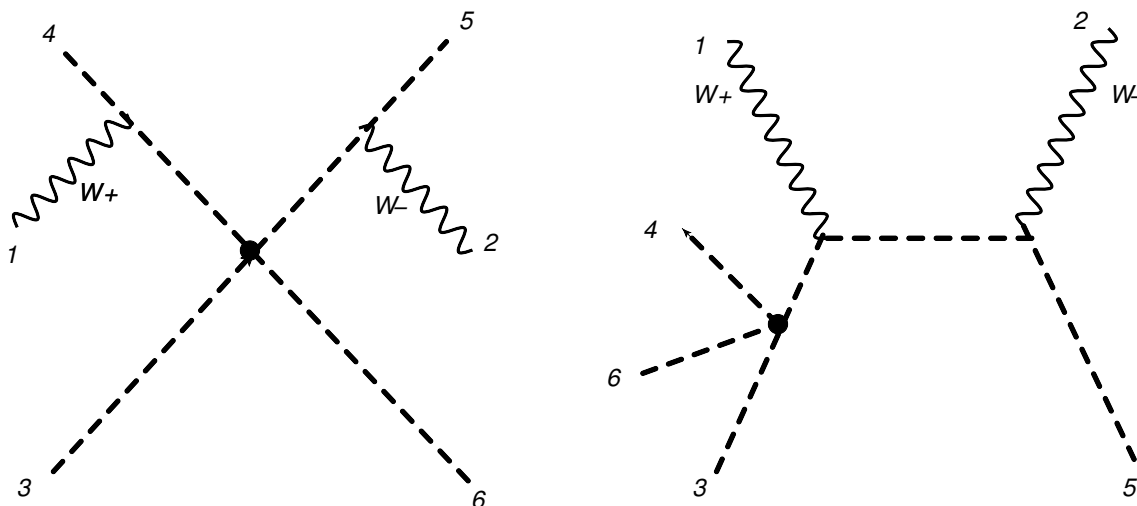
Figure 1. Feynman-diagram of H^2(H^\dagger)^2 WW factorizable amplitude.
