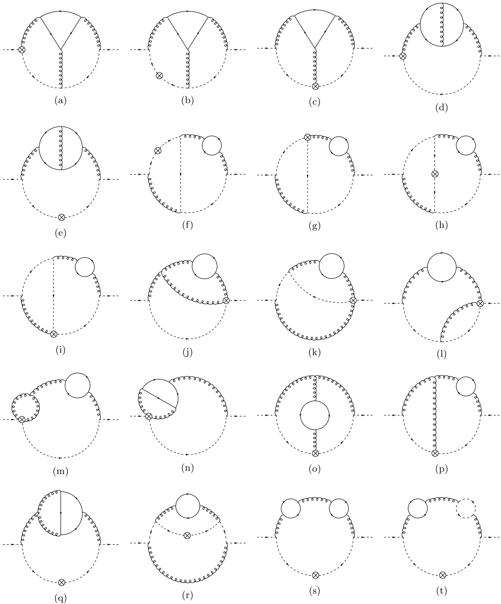
Fig. 2. Sample of diagrams for A_{qq,Q}^{(3),\text{NS}} and A_{qq,Q}^{(3),\text{NS,TR}} . The dashed arrow lines represent massless quarks, while the solid arrow lines represent massive quarks, and curly lines are gluons. The operator insertion Feynman rules for A_{qq,Q}^{(3),\text{NS,TR}} are obtained from those of A_{qq,Q}^{(3),\text{NS}} by making the replacement \not{A} \rightarrow \sigma^{\mu\nu} \Delta_\nu .
