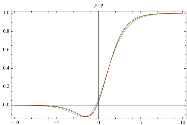
Fig. 1 Temporal variation of \rho + p_r with D = 4 (red), 5 (blue), 10 (green) with A = 1, B\sqrt{\rho_o} = 1
