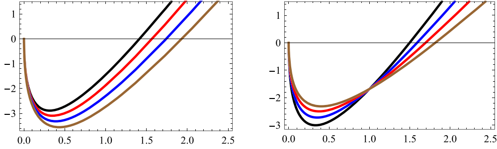
Fig. 1. U(r) versus r for \Lambda = -1 , M = 1 , b = 2.5 , and \nu = -\frac{2}{3} , Eq. (2.16-a). Left: g(\epsilon) = 0.7 and f(\epsilon) = 0.6, 0.78, 0.96, 1.14 for black, blue, red and brown curves, respectively. Right: f(\epsilon) = 0.7 and g(\epsilon) = 0.7, 0.75, 0.8, 0.85 for black, blue, red and brown curves, respectively.
