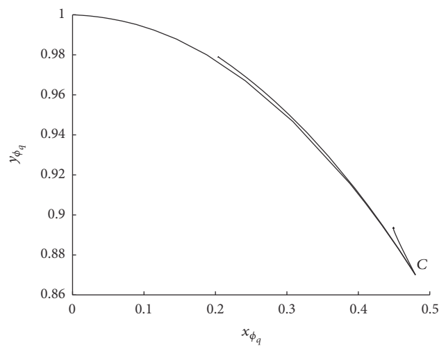
FIGURE 3: Two-dimensional projections of the phase-space trajectories for \beta = 1.5 , \lambda = 0.001 , \lambda = 0.5 , and \lambda = 1.1 . All plots begin from the critical point C = (0.48, 0.87, 0, 0) being a stable attractor.
