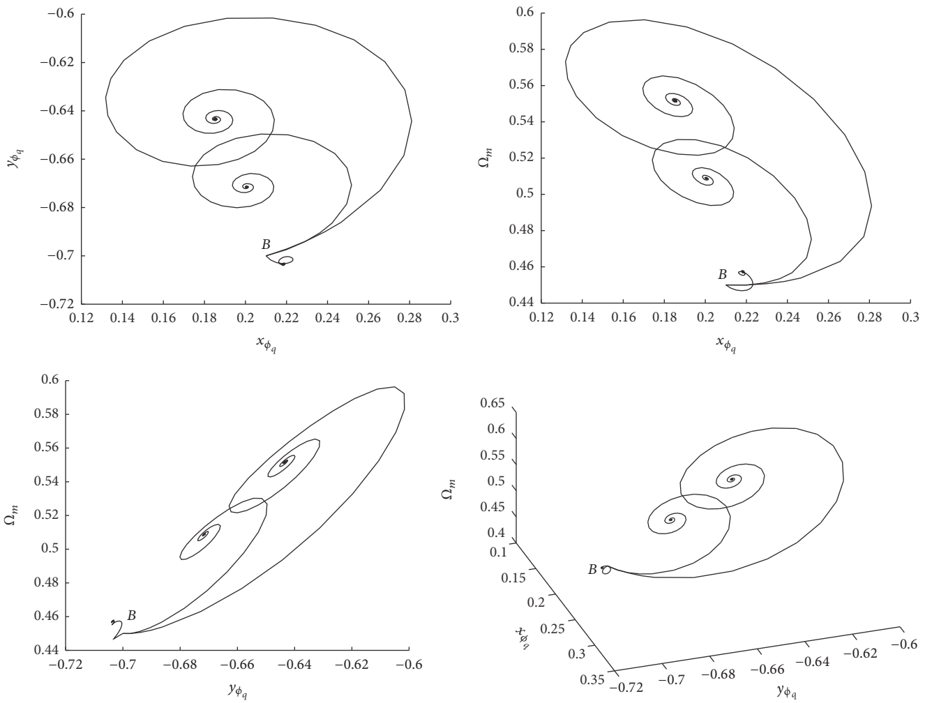
FIGURE 2: Two- and three-dimensional projections of the phase-space trajectories for \beta = 2.51 , \lambda = 3.1 , \lambda = 3.6 , and \lambda = 4.1 . All plots begin from the critical point B = (0.21, -0.70, 0.45, 0) being a stable attractor.
