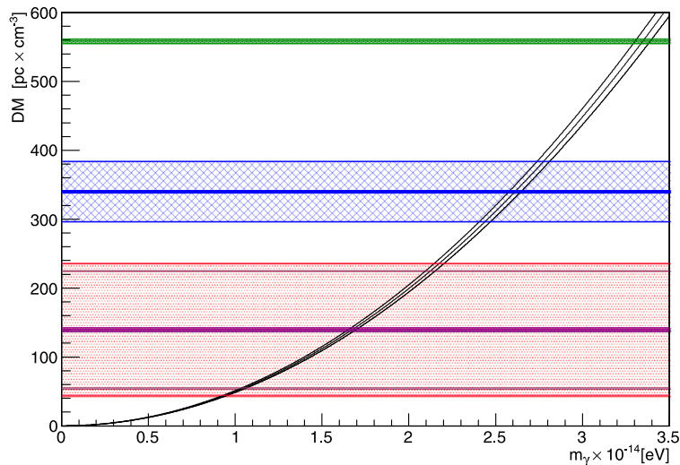
Fig. 1. Contributions to the dispersion measure (DM) budget for FRB 121102. The top (green) band represents the experimental measurement of the total DM = 558.1 \pm 3.3 \text{ pc cm}^{-3} . The middle (blue) band shows the extragalactic contribution, as obtained by subtracting from the central value of the total DM the galactic contribution \text{DM}_{\text{MW}} \equiv \text{DM}_{\text{NE2001}} + \text{DM}_{\text{halo}} = 218 \text{ pc cm}^{-3} [23], to which is assigned an estimated uncertainty of 20%. The bottom (pink) band is obtained by subtracting also the estimated contribution from the intergalactic medium (IGM): \text{DM}_{\text{IGM}} \simeq 200 \text{ pc cm}^{-3} [23], which has an uncertainty of 85 \text{ pc cm}^{-3} associated with inhomogeneities in the IGM, and a smaller uncertainty associated with the cosmological parameters (indicated by the narrow magenta band). The outer pink band shows the total uncertainty in the residual DM after subtraction of \text{DM}_{\text{MW}} and \text{DM}_{\text{IGM}} , with errors added in quadrature. The curved (black) band shows the possible contribution of a non-zero photon mass, m_\gamma , also including the uncertainties in cosmological parameters and the redshift of FRB 121102. (For interpretation of the references to colour in this figure legend, the reader is referred to the web version of this article.)
