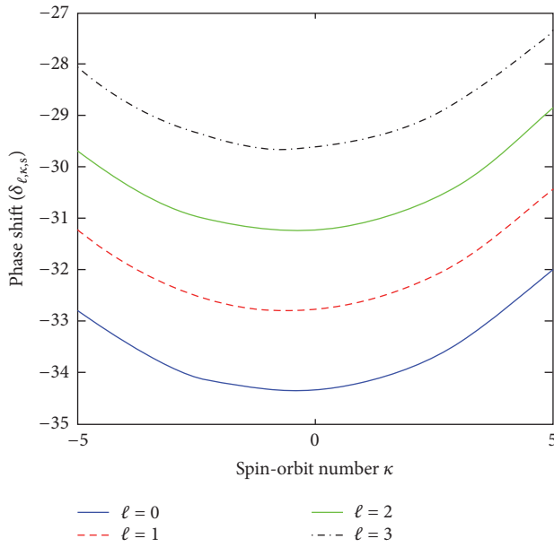
FIGURE 4: A plot of spin scattering phase shifts for the hyperbolic potential as a function of spin-orbit number \kappa for l = 0, 1, 2, 3 with positive potential parameter \sigma_0 = 0.50 , \alpha = 0.50 , c_0 = 1/12 , C_s = 10 , D = 10 , and E = M = 1 . The relativistic mass and energy are equal in all the calculations.
