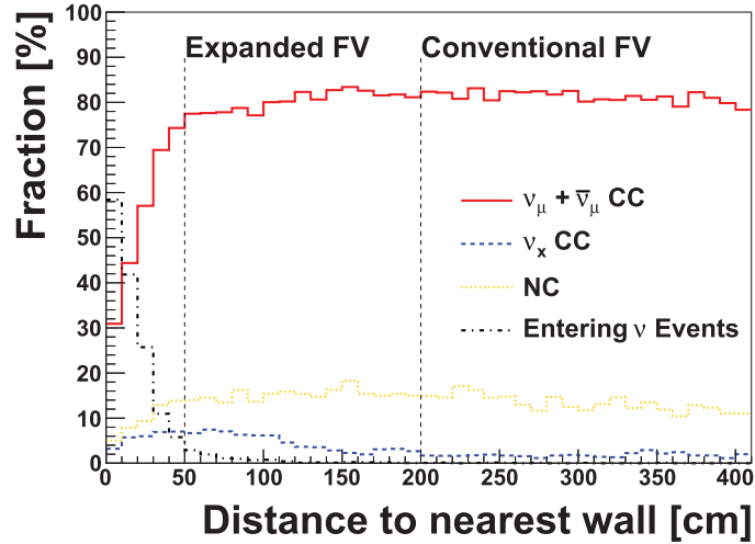
Fig. 11. The fraction of each component of the FC sub-GeV \mu -like 0 decay- e event sample in the atmospheric neutrino MC simulation as a function of the reconstructed distance from the interaction vertex to the nearest wall.
