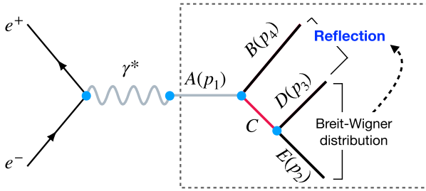
Fig. 1. The schematic diagram for a general three-body process from the electron and positron annihilation. Here, A may denote a vector charmonium or charmoniumlike state with J^{PC} = 1^{--} coupling to a virtual photon. B , D , and E denote the particles involved in the final states, while C is an intermediate state. p_1 , p_2 , p_3 , and p_4 are defined to be the four-momenta of initial state and three final states, respectively, while p_C = p_1 - p_4 corresponds to the propagation momentum of an intermediate C .
