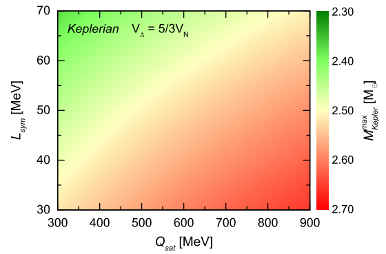
Fig. 5. The maximum masses of Keplerian sequences as a function parameter space spanned by Q_{\text{sat}} and L_{\text{sym}} . The \Delta -resonance potential is fixed at the largest value V_{\Delta} = 5/3V_N considered in this work. The large- Q_{\text{sat}} and small- L_{\text{sym}} range corresponds to compact stars with masses exceeding 2.5 M_{\odot} .
