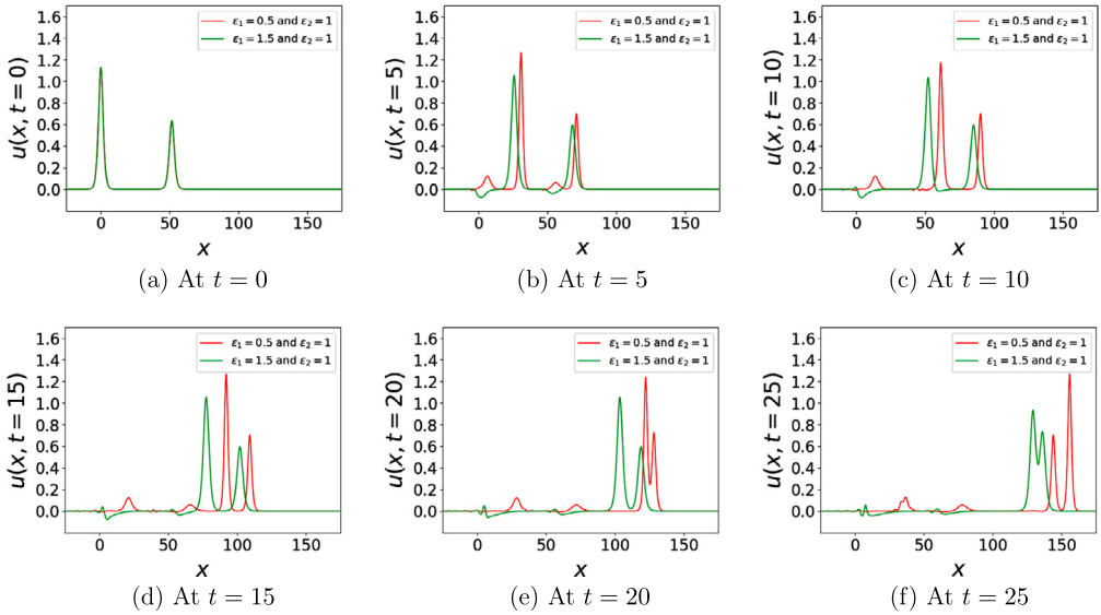
Fig. 20. The time-evolution of two two-soliton systems of equation (1.7) for \varepsilon_1 = 0.5, \varepsilon_2 = 1 (red curve) and \varepsilon_1 = 1.5, \varepsilon_2 = 1 , (green curve) in which the initial conditions were taken from solitons of the mRLW equation.
