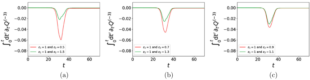
Fig. 14. The time-dependence of the quantity \int_0^t dt' \partial_{t'} Q^{(-3)} as determined in the simulation of equation (1.7), for three-soliton solutions, with \epsilon_1 = 1 and different values of \epsilon_2 \neq 1 .
