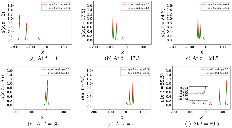
Fig. 12. The time-evolution of two three-soliton systems seen in our simulations of the equation (1.7) with \epsilon_1 = 1 , \epsilon_2 = 0.5 (red curve) and \epsilon_1 = 1 , \epsilon_2 = 1.5 (green curve).
