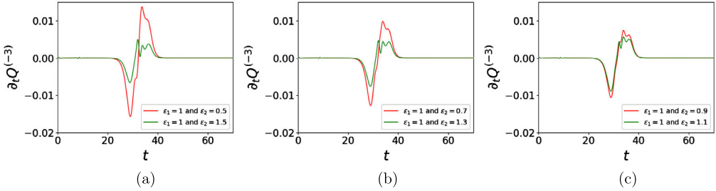
Fig. 13. The time-dependence of \partial_t Q^{(-3)} for a three-soliton system as determined by the simulation of equation (1.7) with \epsilon_1 = 1 and different values of \epsilon_2 \neq 1 .
