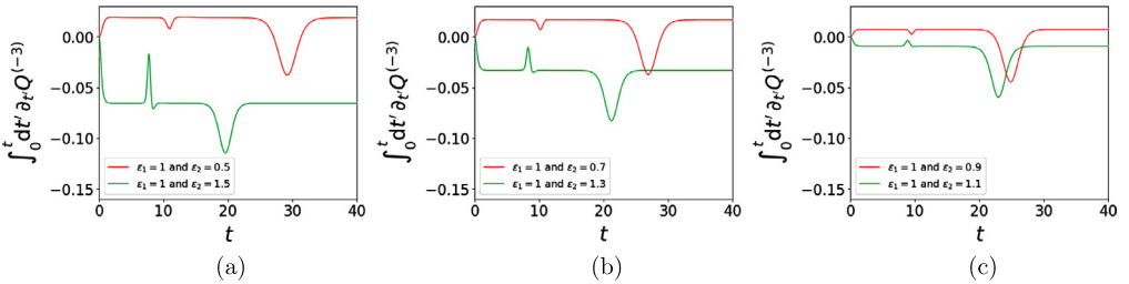
Fig. 19. The time-dependence of \int_0^t dt' \partial_{t'} Q^{(-3)} seen in the simulation of equation (1.7) with different values of \epsilon_1 = 1 and \epsilon_2 \neq 1 .
