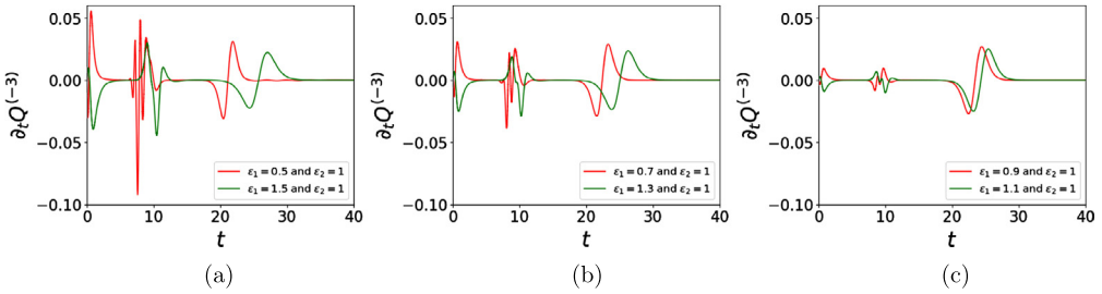
Fig. 21. The time-dependence of the determined values of the quantity \partial_t Q^{(-3)} see in the simulations of equation (1.7) for different values of \varepsilon_1 \neq 1, \varepsilon_2 = 1 .
