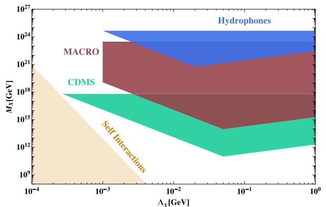
FIG. 5. M_X - \Lambda_\chi parameter space for a fermionic blob, assuming a short-range mediator of mass \mu = \text{TeV} . Both CDMS and hydrophones look for total energy deposition, while MACRO looks for ionization and scintillation signals.
