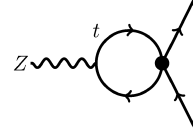
Fig. 1. One loop correction to Z \rightarrow \mu^+\mu^- .
