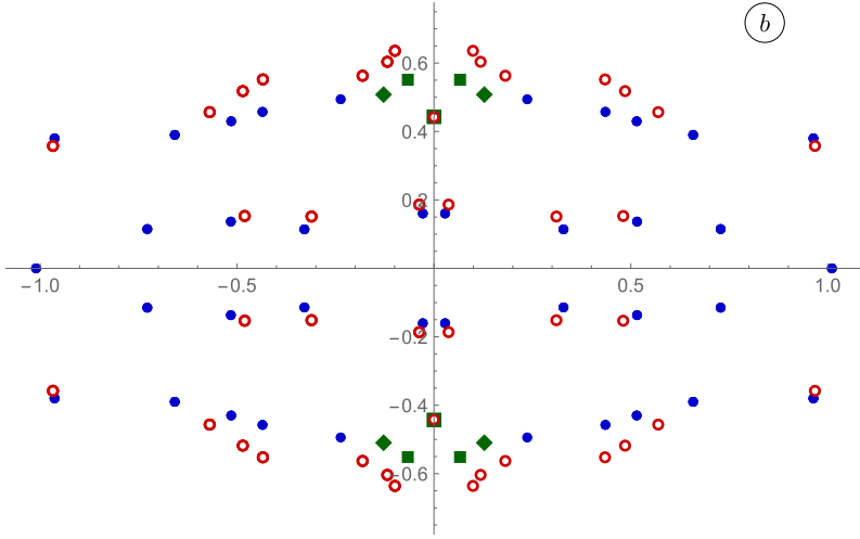
Fig. 15. The open circles depict the distribution of b(N) = \frac{i}{4\pi} \log(B) in the complex plane, where B is the eigenvalue of the quasi-shift operator, for the 42 = 34 + 8 states with L = 3 , \bar{L} = 0 and w = 0 as indicated in Table 1. The filled circles, squares and diamonds correspond to the solutions b_* of eq. (18.14). For the circles \lim_{N \rightarrow \infty} \Im m(b_*(N)) = 0 , while for the squares, b_*(N) \rightarrow \pm \frac{9i}{20} as N \rightarrow \infty . The filled diamonds form two pairs which have the same value of \Im m(b_*(N)) and opposite real part. At large but finite N the diamonds from the upper pair collide at the imaginary axis at which point for one of the diamonds b_*(N) \rightarrow +\frac{9i}{20} while for the other one b_*(N) \rightarrow 0 . The N dependence of b_*(N) for the lower pair of diamonds is obtained from that of the upper pair via complex conjugation.
