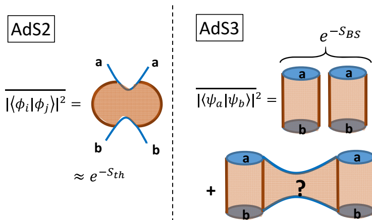
Figure 4. Gravity evaluations of the averages of squares of inner products in AdS 2 gravity (left) and AdS 3 gravity (right).
