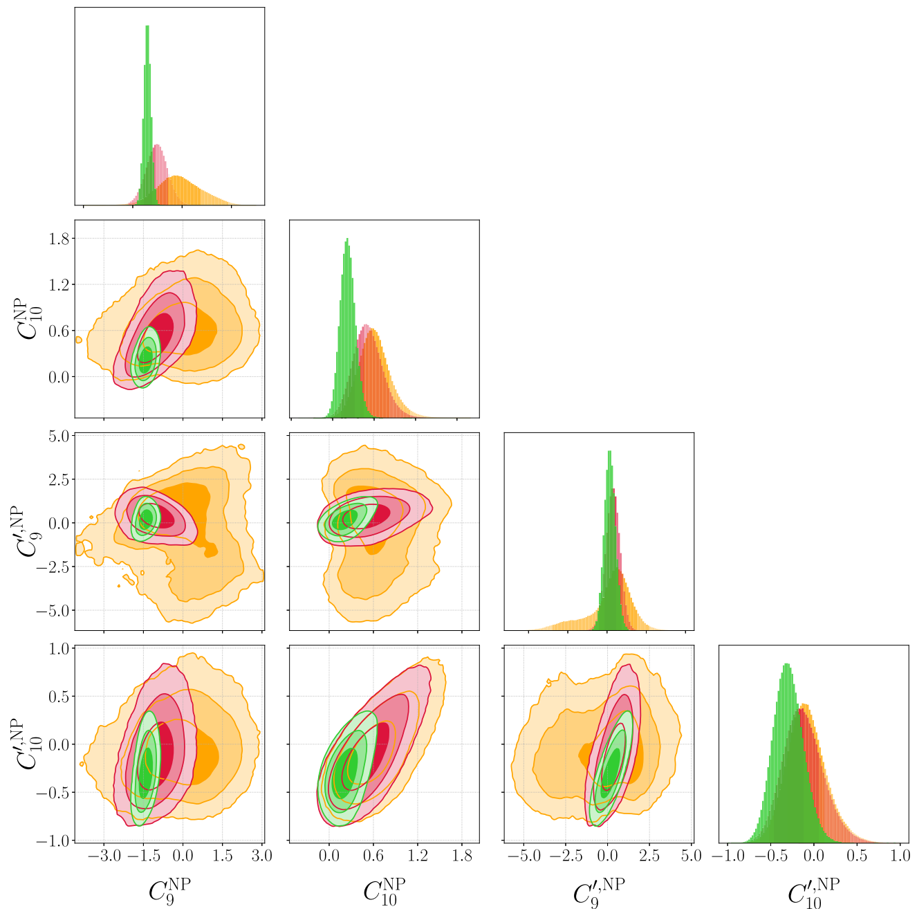
Fig. 8 Posteriors for C_9^{\text{NP}} , C_{10}^{\text{NP}} , C_9'^{\text{NP}} and C_{10}'^{\text{NP}} . Contours and colours as in Fig. 6
