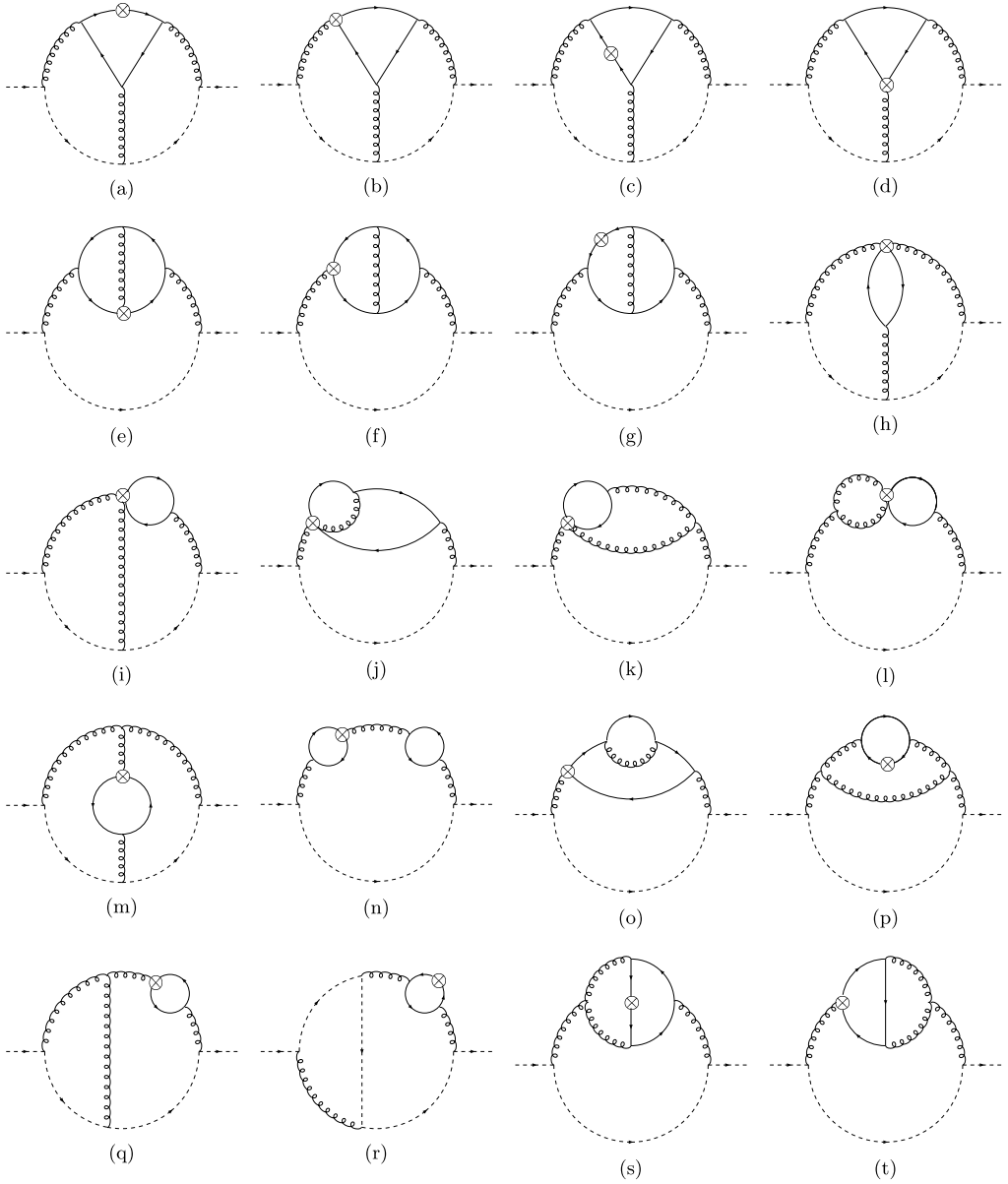
Fig. 1. Sample of diagrams for A_{Oq}^{(3),PS} . The dashed arrow lines represent massless quarks, while the solid arrow lines represent massive quarks, and curly lines are gluons. In terms of Feynman integrals, diagrams (a)–(j) represent the main topologies, in other words, other diagrams, such as diagrams (k)–(t) can be seen as sub-topologies and/or are related to diagrams (a)–(j) by symmetry. The symbol \otimes denotes the local operator insertion, see Ref. [12].
