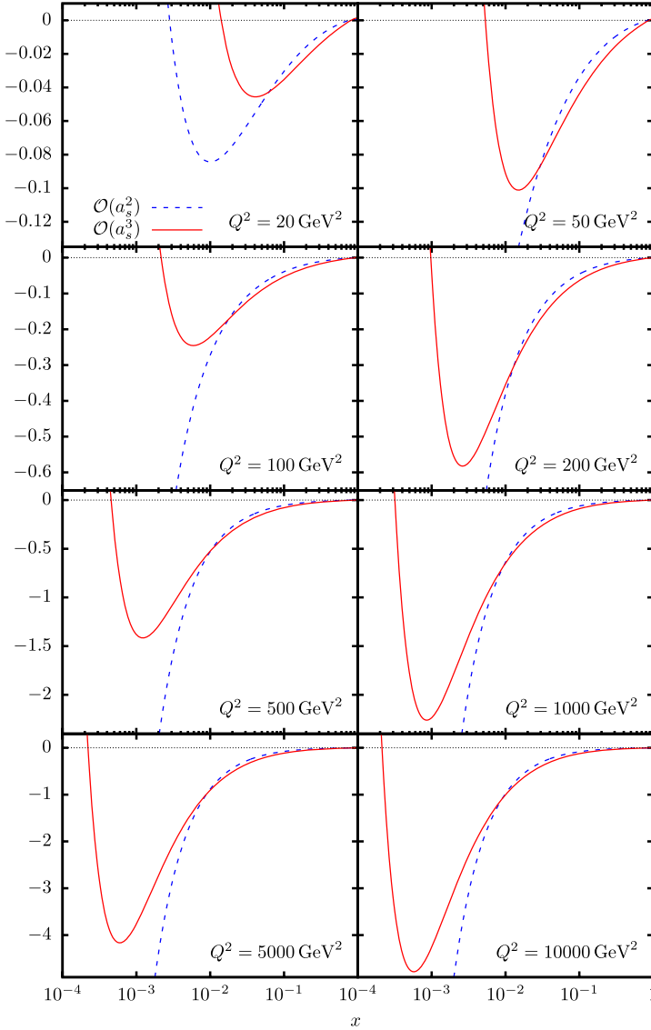
Fig. 9. The Wilson coefficient H_{Q,2}^{\text{PS}} as a function of x and Q^2 choosing Q^2 = \mu^2 and the heavy quark mass m_c = 1.59 GeV (on-shell scheme) at large values of x using the parton distribution functions [4].
