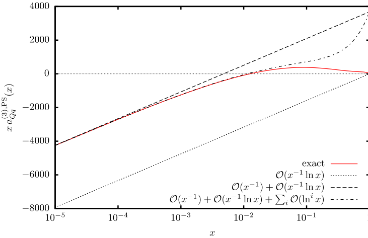
Fig. 4. x a_{Q_q}^{(3),PS}(x) in the low x region (solid red line) and leading terms approximating this quantity; dotted line: ‘leading’ small x approximation O(\ln(x)/x) , dashed line: adding the O(1/x) -term, dash-dotted line: adding all other logarithmic contributions. (For interpretation of the references to color in this figure legend, the reader is referred to the web version of this article.)
