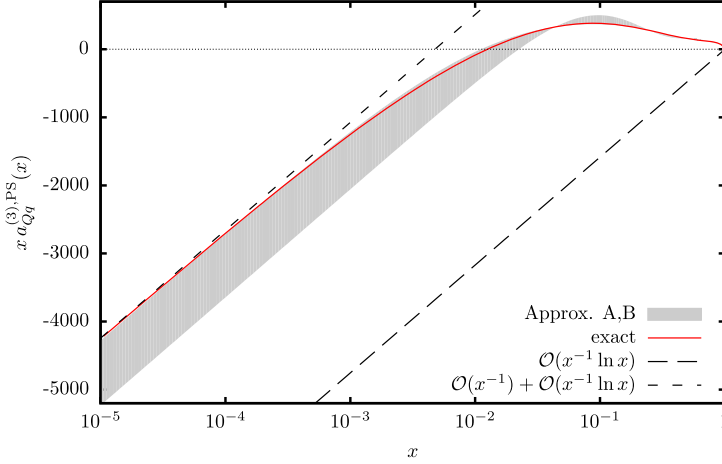
Fig. 5. Comparison of the exact result for x a_{Qq}^{(3),PS}(x) (solid red line) with an estimate in [108] (shaded area). Also shown are the first two leading small x contributions. (For interpretation of the references to color in this figure legend, the reader is referred to the web version of this article.)
