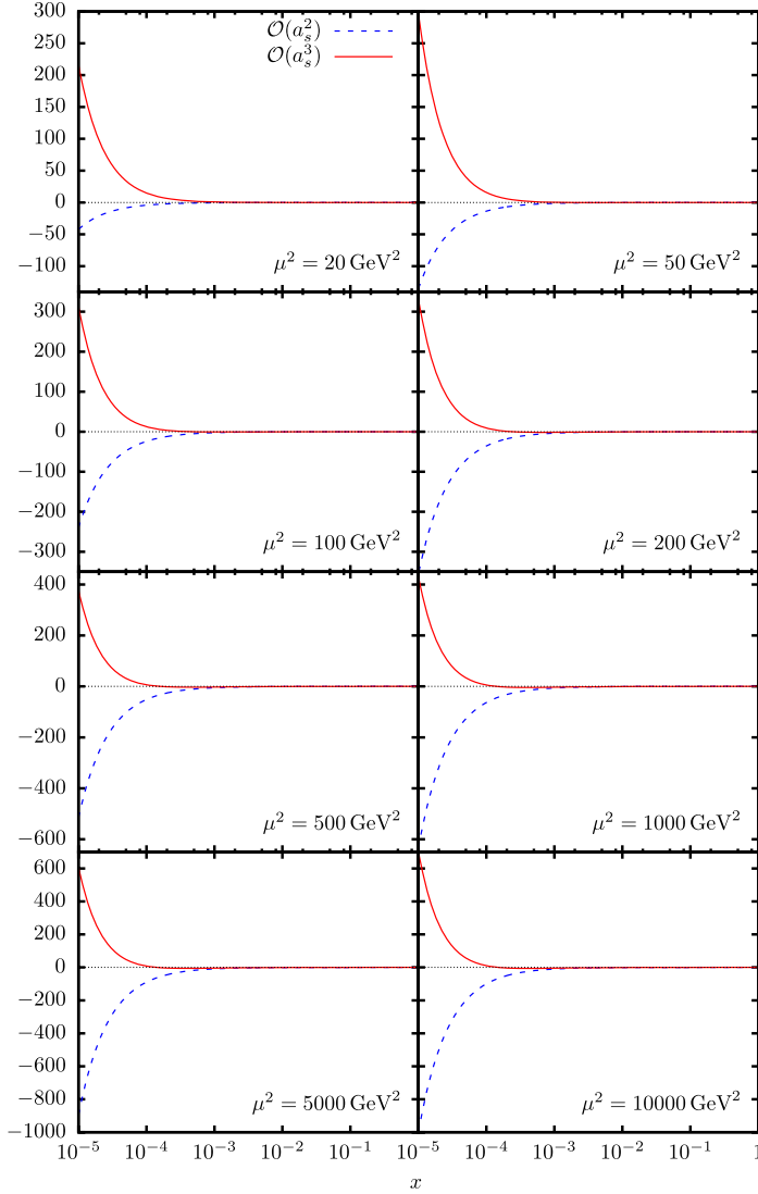
Fig. 6. The OME A_{Oq}^{PS} up to 2- and 3-loop order in dependence of x and \mu^2 for a heavy quark mass m_c = 1.59 GeV (on-shell scheme), cf. [5].
