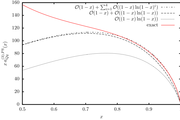
Fig. 3. xa_{Qq}^{(3),PS}(x) in the large x region (solid red line). Dotted line: leading large x behaviour O((1-x)\ln(1-x)) , dashed line: adding the term \propto(1-x) , dash-dotted line: adding all higher logarithms O((1-x)\ln^k(1-x)) . (For interpretation of the references to color in this figure legend, the reader is referred to the web version of this article.)
