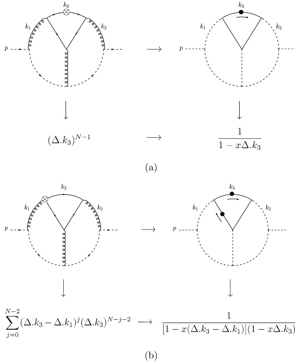
Fig. 2. Graphical illustration of the transformation to the x -representation of the integrals. In (a) we show a line insertion, while in (b) a vertex insertion is depicted. The full circles denote the x -dependent generating functions.
