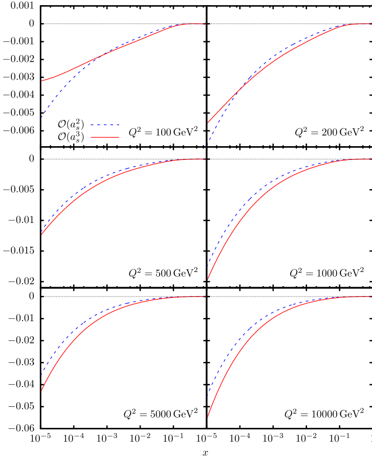
Fig. 11. The bottom contribution by the Wilson coefficient H_{Q,2}^{\text{PS}} to the structure function F_2(x, Q^2) as a function of x and Q^2 choosing Q^2 = \mu^2 , m_b = 4.78 GeV (on shell scheme [112]) using the parton distribution functions [4].
