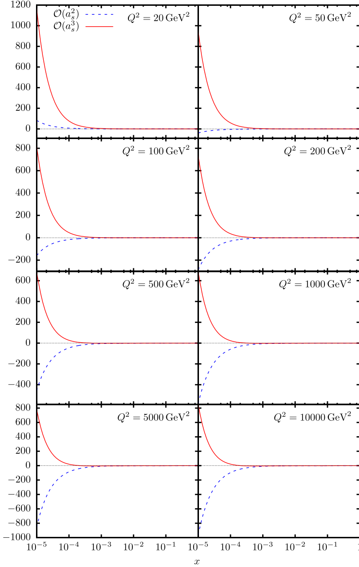
Fig. 8. The Wilson coefficient H_{Q,2}^{\text{PS}} as a function of x and Q^2 choosing Q^2 = \mu^2 and the heavy quark mass m_c = 1.59 GeV (on-shell scheme) using the parton distribution functions [4].
