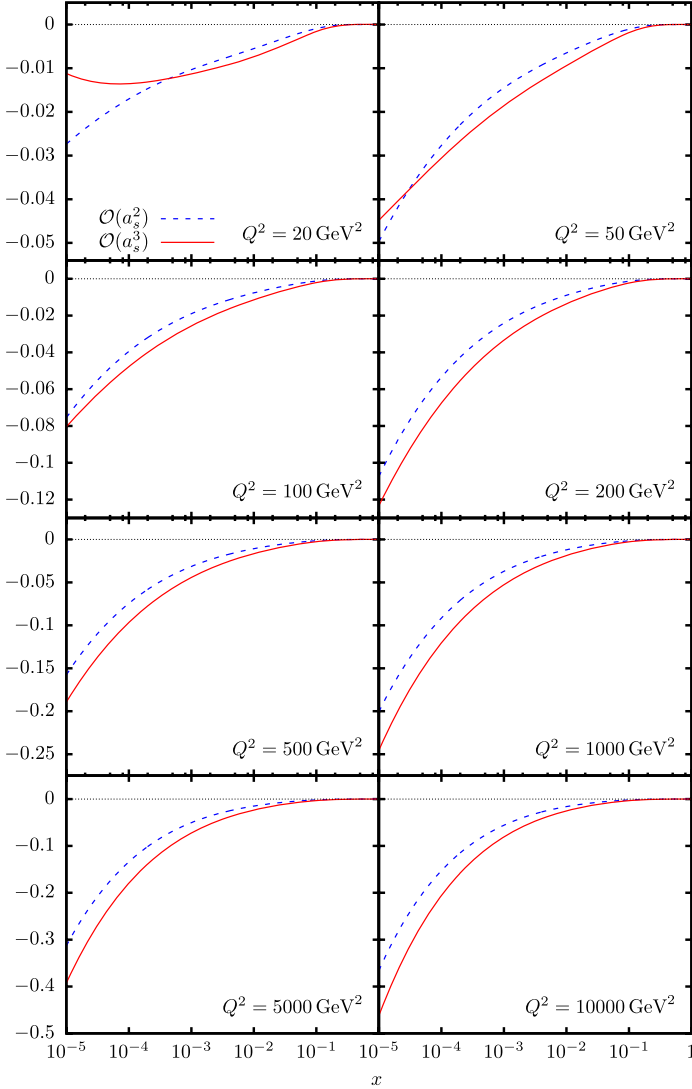
Fig. 10. The charm contribution by the Wilson coefficient H_{Q,2}^{\text{PS}} to the structure function F_2(x, Q^2) as a function of x and Q^2 choosing Q^2 = \mu^2 , m_c = 1.59 GeV (on-shell scheme) using the parton distribution functions [4].
