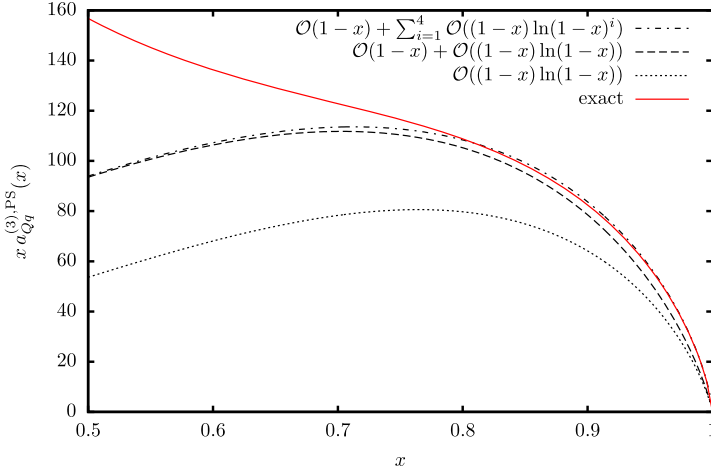
Fig. 3. x a_{Qq}^{(3),PS}(x) in the large x region (solid red line). Dotted line: leading large x behaviour O((1-x)\ln(1-x)) , dashed line: adding the term \propto (1-x) , dash-dotted line: adding all higher logarithms O((1-x)\ln^k(1-x)) . (For interpretation of the references to color in this figure legend, the reader is referred to the web version of this article.)
