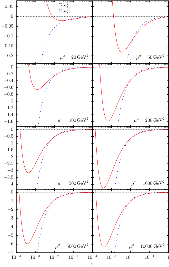
Fig. 7. The OME A_{Qg}^{\text{PS}} up to 2- and 3-loop order in dependence of x and \mu^2 for a heavy quark mass m_c = 1.59 GeV (on-shell scheme) at larger values of x .
