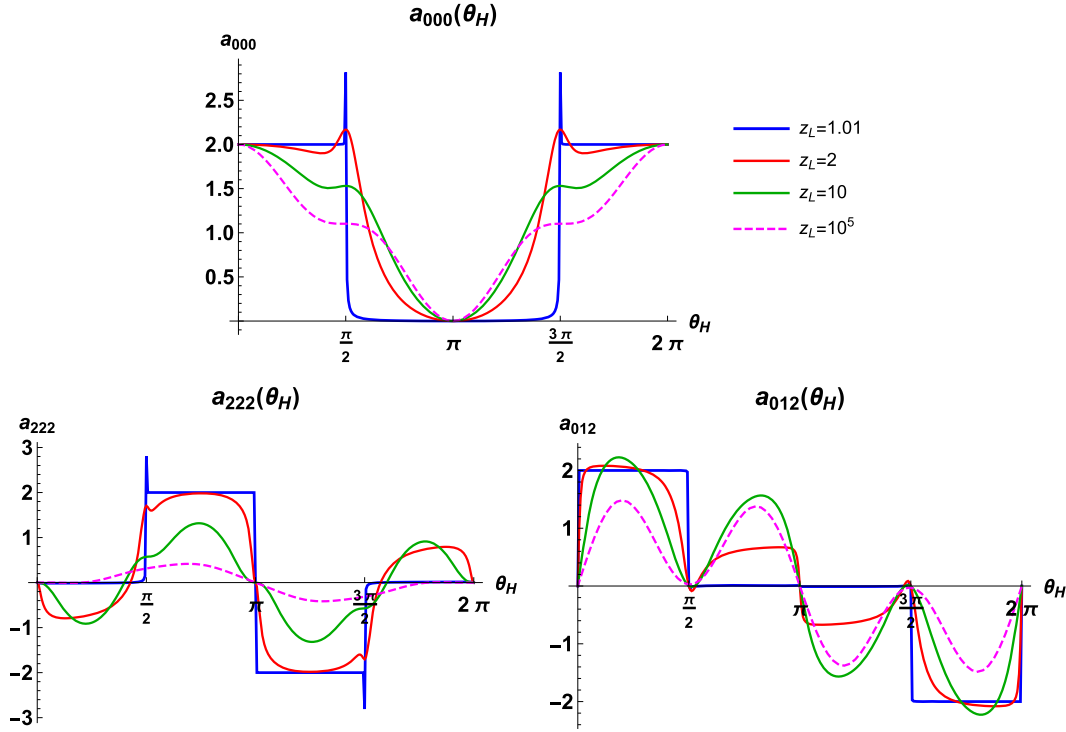
Fig. 9. The anomaly coefficients a_{000}(\theta_H) , a_{222}(\theta_H) , and a_{012}(\theta_H) with c = 0.25 for z_L = 1.01, 2, 10 , and 10^5 . The flat space limit corresponds to k \rightarrow 0 and z_L \rightarrow 1 .
