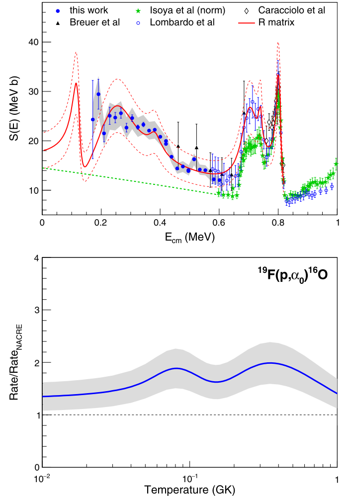
Fig. 4. (Color online.) (Upper panel) S -factor of the ^{19}\text{F}(p,\alpha_0)^{16}\text{O} reaction at low energies ( \lesssim 1 MeV). Blue solid dots: experimental data obtained in this work (error bars: statistical errors; grey band: non-statistical errors). Black triangles: direct data by [10]. Blue empty circles: data by [14]. Green stars: data by Isoya et al. [9] as normalized by NACRE [18]. Black empty diamonds: data by [11]. Green dashed line: non-resonant extrapolation reported in NACRE [18]. Red line: result of R -matrix best-fit of present data and data by Ref. [14]. White band within the red lines: confidence band of the fit. (Lower panel) Reaction rate calculation (expressed as ratio to NACRE) obtained from the R -matrix fit of the S -factor.
