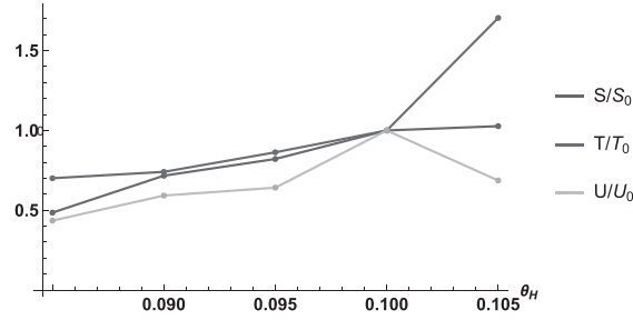
Fig. 1. The \theta_H -dependence of the S, T, U parameters is plotted for m_{\text{KK}} = 13 TeV and n_{\text{max}} = 12 . S_0, T_0, and U_0 are the values of S, T, and U at \theta_H = 0.1 , respectively.
