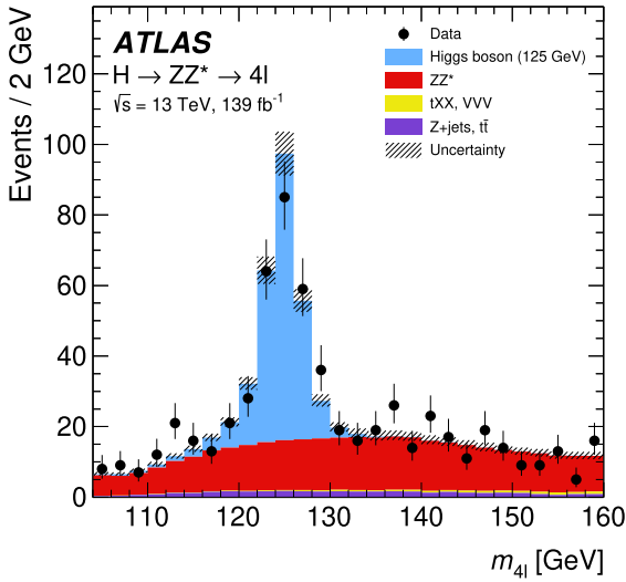
Fig. 2. The observed and expected (pre-fit) m_{4\ell} distributions for the selected Higgs boson candidates. The predicted number of events for these distributions is taken from simulation for the signal, ZZ^* , tXX , and VVV processes, while it is taken from the data-driven estimate (see Section 6) for the Z +jets and t\bar{t} backgrounds. The total uncertainty in the prediction is shown by the hatched band, which also includes the theoretical uncertainties of the SM cross-section for the signal and the ZZ^* background. Higgs boson events in this plot are simulated with m_H = 125 GeV. The p -value quantifying the agreement between the data and MC predictions is 0.36.
