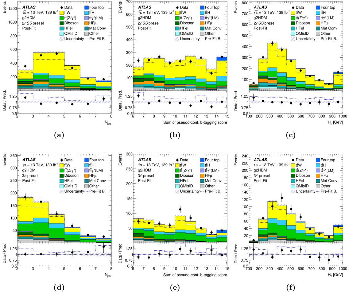
Figure 9. Comparison between data and the background prediction for the distribution of the jet multiplicity (a, d), sum of pseudo-continuous b -tagging scores of jets (b, e) and the sum of p_T of the jets and leptons (c, f), in the 2\ell (a-c) and 3\ell (d-f) signal region selections before any categorisation based on \text{DNN}^{\text{cat}} . The expected signal for m_H = 900 GeV and couplings \rho_{tt}=0.6 , \rho_{tc}=0.0 , and \rho_{tu}=1.1 , along with the background contributions, is shown after the likelihood fit to data (“Post-Fit”) for the background-only hypothesis. The ratio of the data to the prediction (“Pred.”) is shown in the lower panel, separately for post-fit signal-plus-background (black points) and pre-fit background (dashed blue line). The size of the combined statistical and systematic uncertainty in the signal-plus-background prediction is indicated by the blue hatched band. The last bin in each figure contains the overflow.
