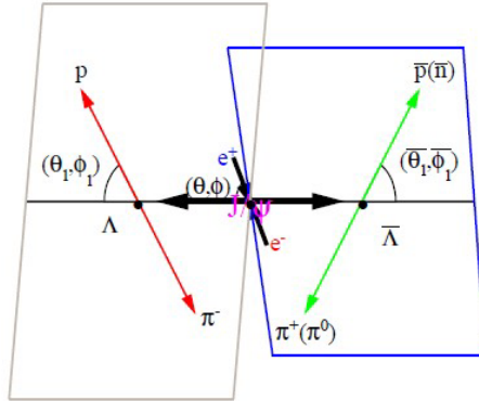
Fig. 1. Definition of the helicity frame for J/\psi \rightarrow \Lambda \bar{\Lambda} , \Lambda \rightarrow B\pi , \bar{\Lambda} \rightarrow \bar{B}\pi .
