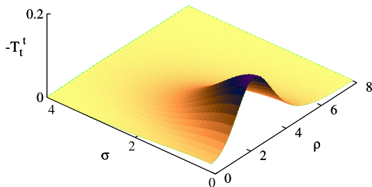
Fig. 2. The T_t^t -component of the energy momentum tensor is shown as a function of the coordinates \rho = r \sin \theta , \sigma = \rho \cos \theta , for a nodeless boson star with m = 1 , w/\mu = 0.93 . Here, T_t^t , \rho and \sigma are given in units of the scalar field mass \mu .
