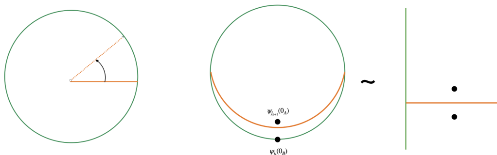
Figure 3. Two kinds of Euclidean time on the disk. Left: Euclidean Rindler time, defined in eq. (3.40). We will use this when we construct the dS/AdS wormhole by gluing (two copies of) disk and Euclidean de Sitter in section 3.4. Right: the global time on the disk induced from the time on a Euclidean strip. Black dots represent operators on the dS/AdS wormhole as in eq. (3.9).
