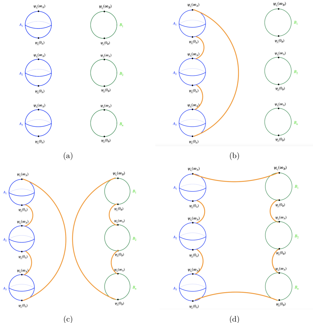
Figure 1. Possible gravitational saddles of the n = 3 Rényi entropy (2.3) connecting copies of the universes A (de Sitter) and B (an AdS black hole). (a) Totally disconnected saddle where all copies of A and B are disconnected. (b) Type II_A configuration where all copies of the universe A are connected by a replica wormhole, but the copies of the universe B are disconnected. In the same way, we have Type II_B configurations where all copies of universe B are connected by a replica wormhole. (c) In the Type III configuration, each copy of A is linked by a replica wormhole, and each copy of B is linked by a separate replica wormhole, but the two wormholes are not interconnected. (d) In a Type IV configuration, all copies are connected through a single wormhole.
