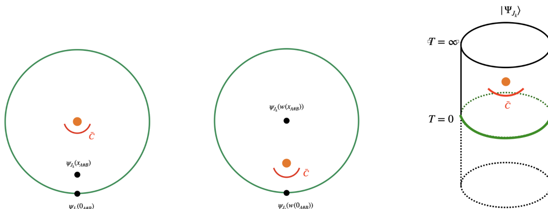
Figure 10. Sequence of two dimensional surfaces used to compute the CFT sum (4.16). Left: z disk on which the correlation functions in (4.16) are originally defined. The cosmological horizon is depicted by the orange dot at the center, and the endpoints of the cut \bar{C} are located near the horizon. Center: w disk on which one of the operators are located at the center of this disk. The w and z disks are related by the map (4.17). Right: the w disk is mapped to the T > 0 part of the cylinder by an exponential map. The operator at the center of the w disk is now at T = \infty and represented by an excited state |\psi_{J_k}\rangle by the state operator correspondence. The T < 0 part of the cylinder is provided by the copy of the w disk, which naturally emerges when we compute the correlation function on the disk by the doubling trick as in eq. (4.21). This results in the same excited state |\psi_{J_k}\rangle appearing at T = -\infty as well. In the cylinder frame, eq. (4.21) has an interpretation as a Rényi entropy, as in eq. (4.25).
