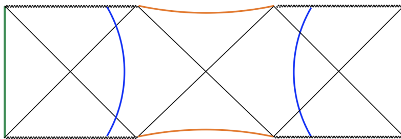
Figure 5. The Lorentzian spacetime on which we compute the generalized entropy (in eq. (4.11)). This spacetime is obtained by continuing the Euclidean wormhole geometry to Lorentzian signature along the reflection symmetric slice. This is an asymptotically AdS black hole (whose conformal boundaries are depicted in green) with an inflating de Sitter region in its interior (with future and past infinities depicted in orange curves). The blue curves represent domain walls separating two geometries.
