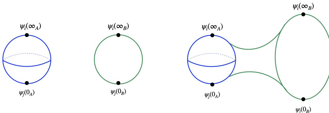
Figure 6. Left: the path integral preparations of overlaps \langle \psi_i | \psi_j \rangle_A and \langle \psi_i | \psi_j \rangle_B computed in Euclidean de Sitter (blue) and AdS black hole (green) spacetimes. They appear in quantity (2.3) of our interest. The excited states are specified by inserting corresponding operators. Right: Euclidean de Sitter and AdS black hole spacetimes are connected by a wormhole. Such a wormhole appears, for example, in the gravitational path integral (2.4) for the normalization of the reduced density matrix. We have already constructed this dS/AdS wormhole solution in JT gravity in section 3.4.
