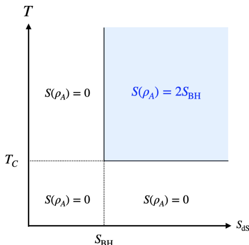
Figure 11. Phase diagram for the entanglement entropy S(\rho_A) (which is equal to S(\rho_B) as the entire state is pure). In drawing this diagram, we fix the entropy of the AdS black hole and change the entanglement temperature and the de Sitter entropy. The entanglement entropy is non-vanishing only when S_{\text{dS}} > S_{\text{BH}} and temperature is large, where the fully connected saddle dominates the gravitational path integral for the Rényi entropy.
