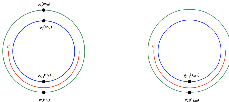
Figure 8. Left: each of the replica copies in the fully connected wormhole depicted in figure 7 with four operator insertions, connected by cut C (the red line). The contribution from this wormhole appears in the quantity of our interest, \text{tr} \rho_A^n in eq. (2.3), and is given by eq. (4.1). The blue circle is the greater circle of the original Euclidean de Sitter space with two operator insertions \psi_{i_k}(\infty_A) and \psi_{j_{k+1}}(0_A) . Right: the operator configuration in the same geometry after taking the OPE \psi_{i_k}(\infty_{A_k}) \rightarrow \psi_{i_k}(\infty_{B_k}) and factoring the corresponding component, which is suppressed. By summing over the leftover indices, this leads to eq. (4.8).
