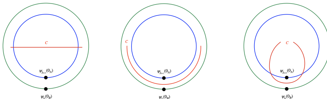
Figure 9. Three possible cuts C for the fully connected wormhole \mathcal{M}_n which contributes to the gravitational path integral for the Rényi entropy as in eq. (4.8). Left: type A cut located above two operators. Since two operators in the disk are not always the same, this type of cuts only gives a subdominant contribution to the gravitational path integral (4.2). Center: type B cut whose endpoints are located near the bifurcation surfaces of the AdS black hole. Right: type B cut which ends near the cosmological horizon. One of the purposes of this subsection is to argue that the endpoints of the cut of this type are not precisely on the cosmological horizon. (If they were, it would result in a vanishing entropy S(\rho_A) = 0 .)
