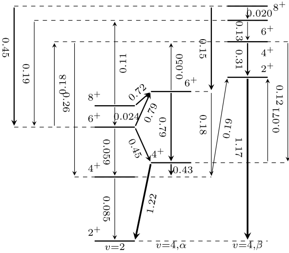
Fig. 1. The E2 transition strengths relative to B(E2; 2_1^+ \rightarrow 0_1^+) (denoted as B_{20} ) for a system with four particles (holes) in j = 9/2 shell calculated using a seniority-conserving interaction. The 0_1^+ states and few weakest transitions are not shown for simplicity. One has B(E2; 2_1^+ \rightarrow 0_2^+) = 0.044B_{20} and B(E2; 2_2^+ \rightarrow 0_2^+) = 0.19B_{20} . The two v = 4, \alpha states do not mix with others for any g_{9/2} interaction.
