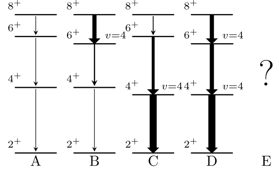
Fig. 2. Illustration on E2 transitions for the yrast states of a (9/2)^4 system in different scenarios based on E2 transitions from Fig. 1: A. All lowest excited states are dominated by seniority v = 2 configurations with suppressed E2 transitions below them; B. The special v = 4, 6^+ state becomes yrast with a large B(E2; 8_1^+ \rightarrow 6_1^+) value, in which situation the 8_1^+ state may not be isomeric; C. Similar to B but with the special v = 4, 4^+ state becomes yrast; D. Both special v = 4, 4^+ and 6^+ states become yrast where a collective-like strong inband E2 transition pattern is formed. E. One may wonder if it is possible to have a strong mixture between the v = 2 and 4 states (see text for details).
