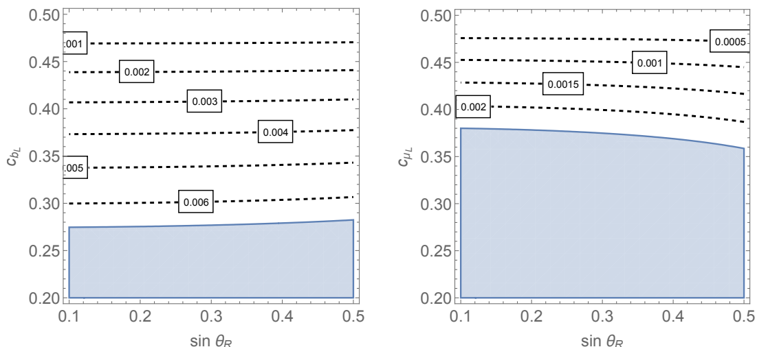
Figure 8. Left panel: contour lines of \delta g_{Z_L b_L b_L} in the plane (\sin \theta_R, c_{b_L}) where we have fixed \sin \theta_\Sigma = 0.72 . The white region is allowed by electroweak precision data at the 95% CL. Right panel: the same for \delta g_{Z_L \mu_L \mu_L} .
