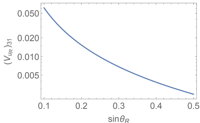
Figure 5. Upper bound on (V_{u_R})_{31} as a function of \sin \theta_R from condition (4.29) for m_1=3 TeV, using the value of (V_{u_R}^\dagger)_{23} provided by R_{D^{(*)}} .
