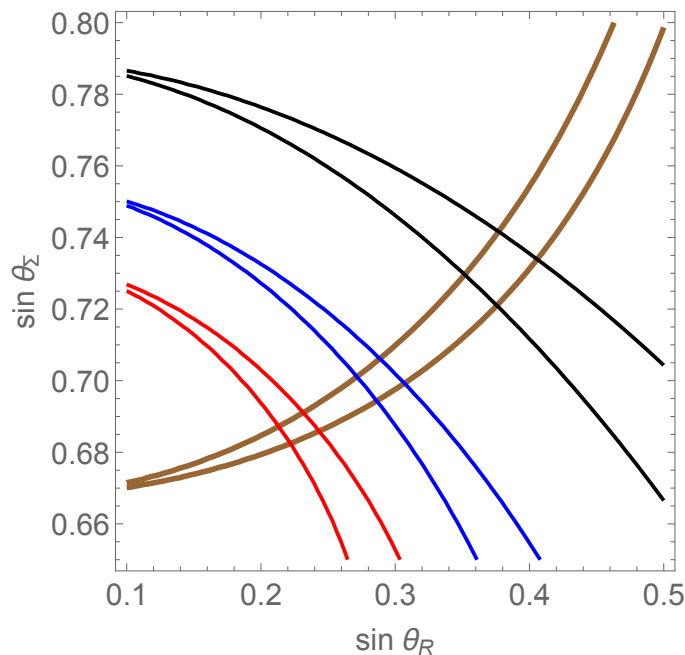
Figure 3. The region between the solid lines is allowed by \delta g_{Z_L \tau_R \tau_R} (brown lines, as obtained in figure 2) and by the 95 % C.L. bound on the T parameter, for m_1 = 3 TeV and \tan \beta = 1 (black lines), \tan \beta = 3 (blue lines) and \tan \beta = 5 (red lines).
