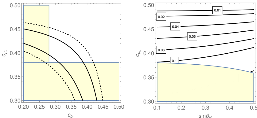
Figure 12. Left panel: contour lines of constant \Delta C_{LL}^\mu in the plane (c_{b_L}, c_{\mu_L}) using V_{d_L} \simeq V , at 1 \sigma (solid lines) and 2 \sigma (dashed lines) level as defined in eq. (5.24). The value of \sin \theta_R = 0.35 has been fixed. Right panel: contour lines of constant \Delta C_{RL}^\mu in the plane (\sin \theta_R, c_{\mu_L}) after selecting the upper bound on |(V_{d_R}^\dagger)_{23}| \simeq 0.005 obtained in eq. (4.32). In both panels the shaded yellow area corresponds to the excluded area obtained in figure 8.
