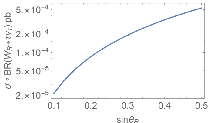
Figure 7. Plot of \sigma(pp \rightarrow W_R^1) \times \mathcal{B}(W_R^1 \rightarrow \tau_R \nu_{\tau_R}) as a function of \sin\theta_R , for m_1 = 3 TeV and the values of (V_{u_R}^\dagger)_{23} required for the solution to the R_D^{(*)} anomaly.
