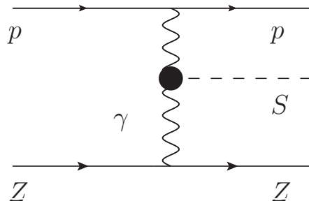
Figure 20. A diagram of the production of a scalar in photon fusion.
