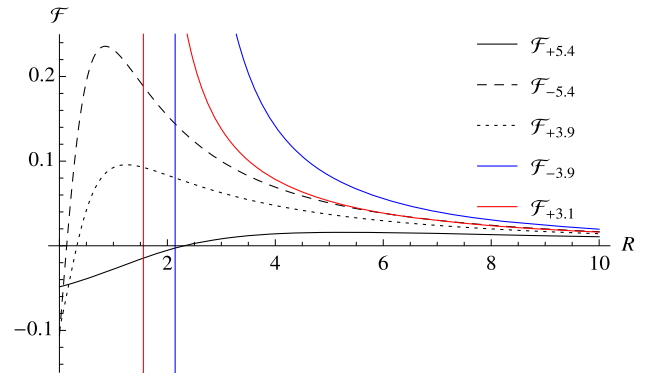
Fig. 3. The behavior of the interaction force for M_1 = 1 , M_2 = 2 , a_1 = 1.5 , and several angular momentum values per unit mass a_2 labeled with a subindex. The merger limit is indicated by a vertical asymptote.
