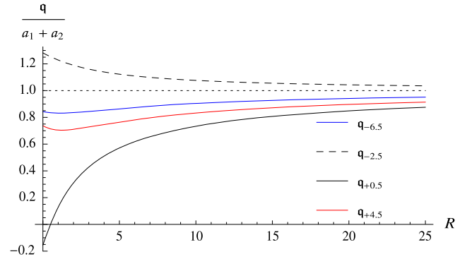
Fig. 2. Several figures of q in the unequal case, for M_1 = 1 , M_2 = 2 , a_1 = 1.5 , and different angular momentum values per unit mass a_2 indicated by the subindex.
