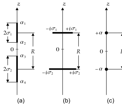
Fig. 1. Schematic representation of different types of unequal Kerr sources: (a) BH configuration \sigma_i^2 > 0 ; (b) hyperextreme sources if \sigma_i \rightarrow i\sigma_i (or \sigma_i^2 < 0 ); (c) the extreme limit case \sigma_i = 0 .
