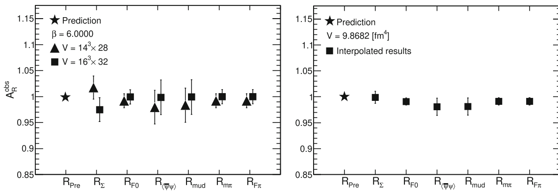
Fig. 19 Comparing the prediction with the fitting results of the slopes A_R^{obs} to the ratios R_{obs} . The configurations of V = 14^3 \times 28 and V = 16^3 \times 32 of \beta = 6.0000 (left) and the interpolated results (right)
