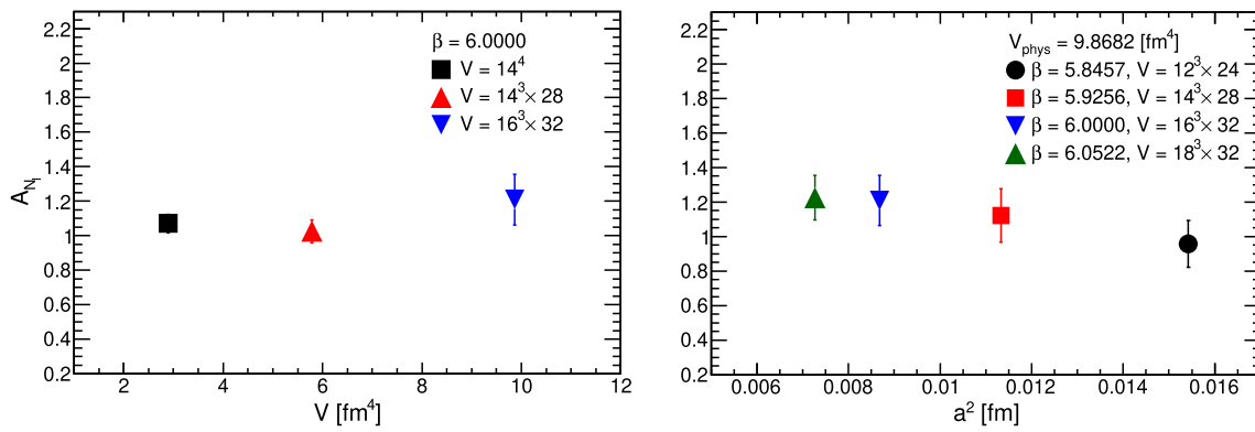
Fig. 7 Examining the effects of the finite lattice volume (left) and the discretization (right) on the fitting results of the slope A_{N_l} . The outcomes of \beta = 6.0000 , V = 14^4 and \beta = 6.0522 , V = 18^3 \times 32 are reported in our previous research [41,42]
