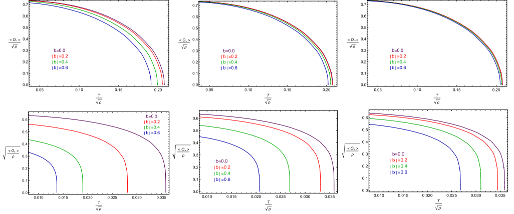
Fig. 1. (Color online) The condensation operators \mathcal{O}_- and \mathcal{O}_+ with the ENE (left two panels), BINE (middle two panels) and LNE (right two panels) in terms of temperature in the backreacted holographic superconductor model for d = 4 dimension and the mass of the scalar field m^2 = -2 . In each panel, the various colors represent different value of the nonlinear parameter, i.e. |b| = 0 (purple), 0.2 (red), 0.4 (green) and 0.6 (blue) respectively.
