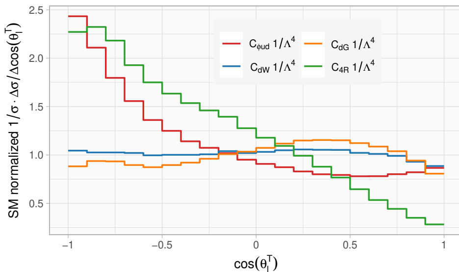
Figure 26. To itself and to the SM normalized SMEFT contributions to the \cos \theta_l^T distribution at NLO in QCD. Results are presented for Q_{\varphi ud}^{33} , Q_{dW}^{33} and Q_{dG}^{33} as well as for the four quark operator Q_{4R} .
