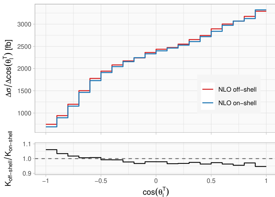
Figure 17. Distribution of \cos \theta_l^T at NLO in the on-shell approximation and for an off-shell top quark. The lower panel shows the ratio of the off-shell and on-shell K -factors. Note the range of the y -axis, which does not start at zero.
