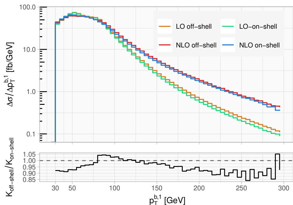
Figure 6. Leading b -jet transverse momentum distributions for the top-quark on-shell approximation and for the off-shell top quark at LO and NLO. The lower panel shows the ratio of the NLO/LO K -factors from the off-shell and on-shell results.
