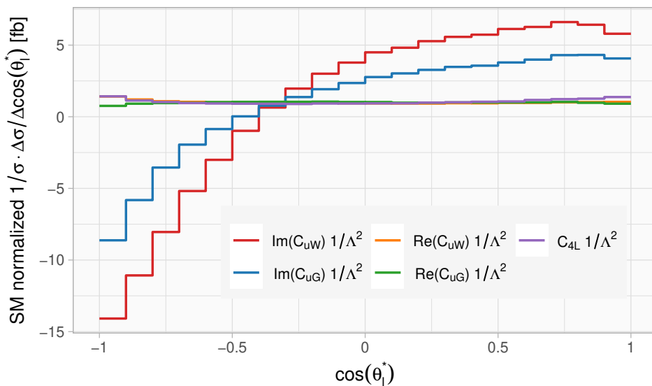
Figure 22. To itself and to the SM normalized SMEFT contributions to the \cos\theta_l^* distribution at NLO in QCD. Results are presented for the real and imaginary parts of C_{uW}^{33} and C_{uG}^{33} as well as for the four quark operator C_{4L} .
