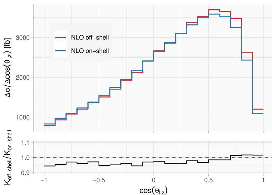
Figure 16. Distribution of \cos \theta_{l,z} at NLO in the on-shell approximation and for an off-shell top quark. The lower panel shows the ratio of the off-shell and on-shell K -factors. Note the range of the y -axis, which does not start at zero.
