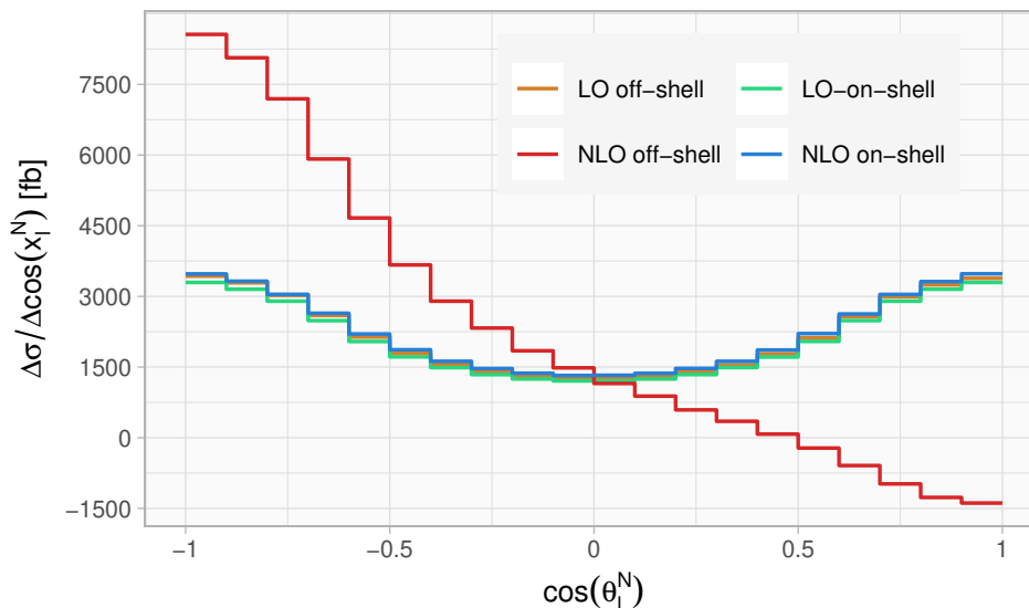
Figure 8. Angular distribution \cos \theta_1^N at LO and NLO for an on-shell and off-shell top quark. The NLO off-shell result becomes unphysical and indicates a strong sensitivity to the cancellation of soft radiation.
