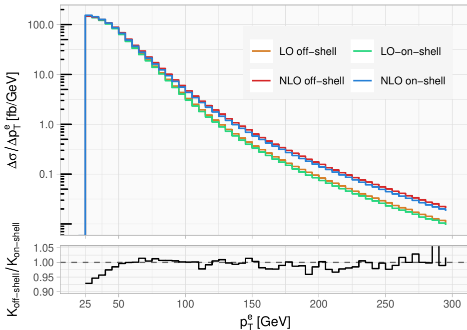
Figure 5. Positron transverse momentum distributions for the top-quark on-shell approximation and for the off-shell top quark at LO and NLO. The lower panel shows the ratio of the NLO/LO K -factors from the off-shell and on-shell results.
