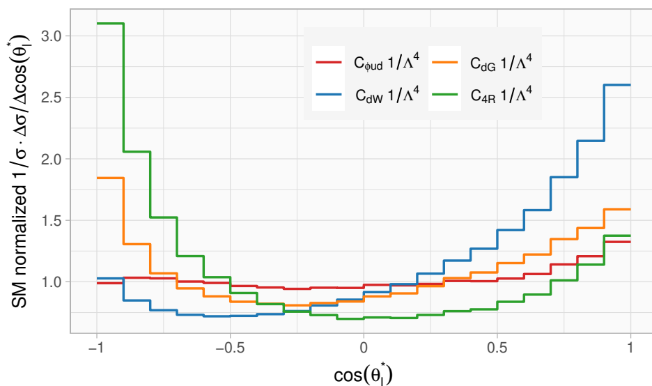
Figure 27. To itself and to the SM normalized SMEFT contributions to the \cos \theta_l^* distribution at NLO in QCD. Results are presented for Q_{\varphi ud}^{33} , Q_{dW}^{33} and Q_{dG}^{33} as well as for the four quark operator Q_{4R} .
