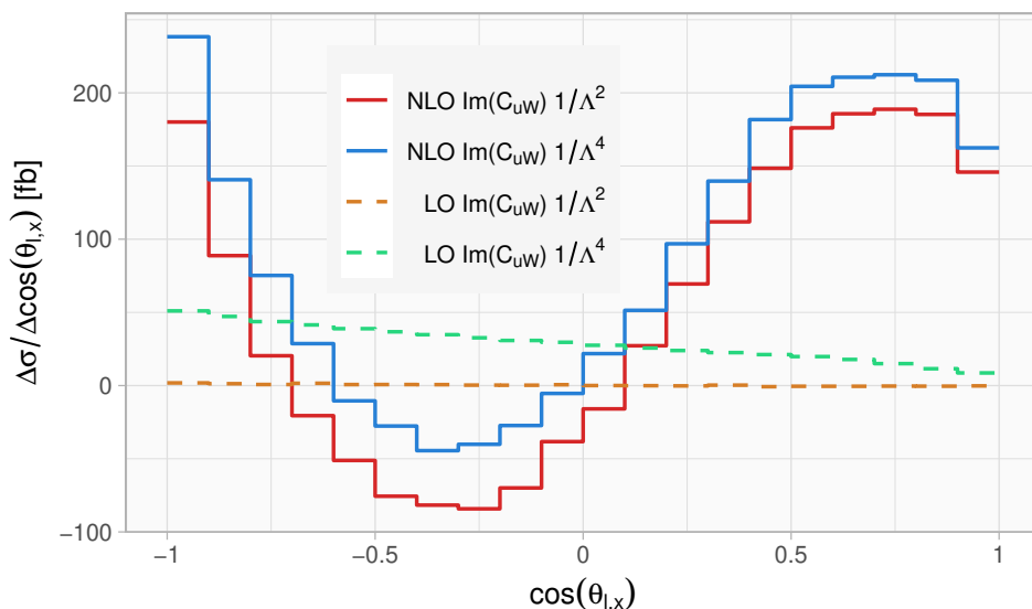
Figure 11. Distribution of \cos\theta_{l,x} for the pure SMEFT contribution with \Im m C_{uW}^{33} = 1 , \Lambda = 1000\text{ GeV} . Shown are results at LO and NLO in QCD and at 1/\Lambda^2 in the SMEFT as well as higher order effects 1/\Lambda^4 .
