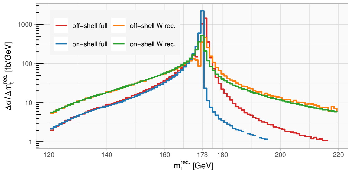
Figure 4. Reconstructed top-quark mass distribution for an on-shell and off-shell top quark at NLO. The full result denotes reconstruction through the full W -boson and b -jet four vectors. The “W rec.” lines denote the reconstruction of the neutrino’s longitudinal component.
