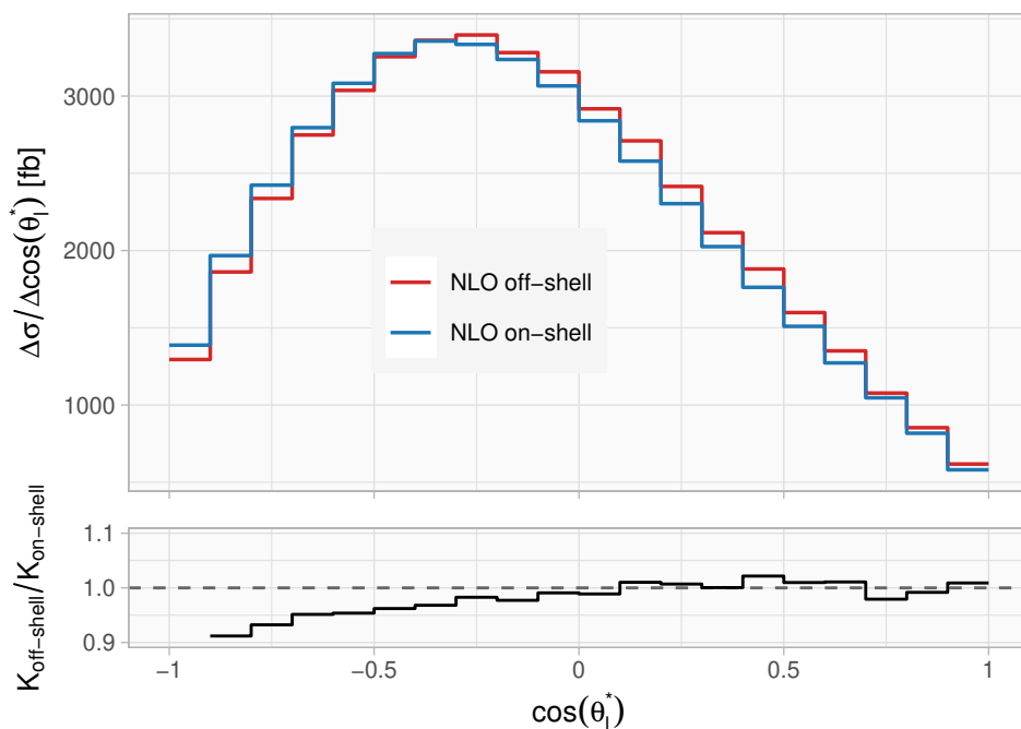
Figure 18. Distribution of \cos \theta_i^* at NLO in the on-shell approximation and for an off-shell top quark. The lower panel shows the ratio of the off-shell and on-shell K -factors. Note the range of the y -axis, which does not start at zero.
