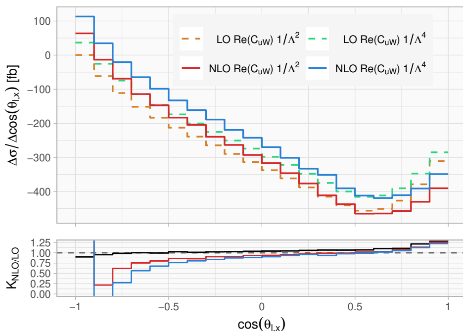
Figure 9. Distribution of \cos\theta_{l,x} for the pure SMEFT contribution with \Re c_{uW}^{33} = 1 , \Lambda = 1000 GeV. Shown are results at LO and NLO in QCD and at 1/\Lambda^2 in the SMEFT as well as with higher order effects 1/\Lambda^4 .
