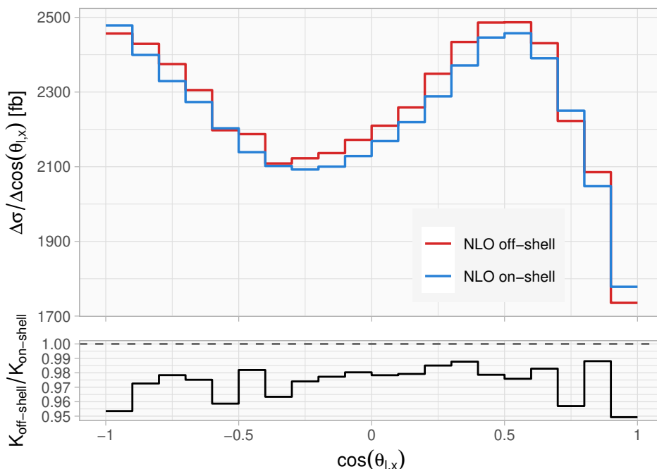
Figure 14. Distribution of \cos \theta_{l,x} at NLO in the on-shell approximation and for an off-shell top quark. The lower panel shows the ratio of the off-shell and on-shell K -factors. Note the range of the y -axis, which does not start at zero.
