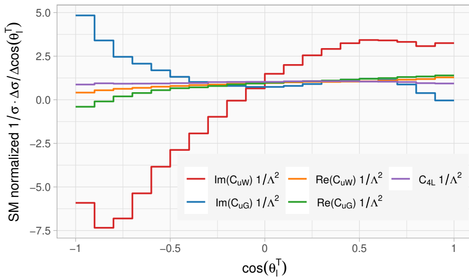
Figure 21. To itself and to the SM normalized SMEFT contributions to the \cos \theta_l^T distribution at NLO in QCD. Results are presented for the real and imaginary parts of \mathcal{C}_{uW}^{33} and \mathcal{C}_{uG}^{33} as well as for the four quark operator \mathcal{C}_{4L} .
