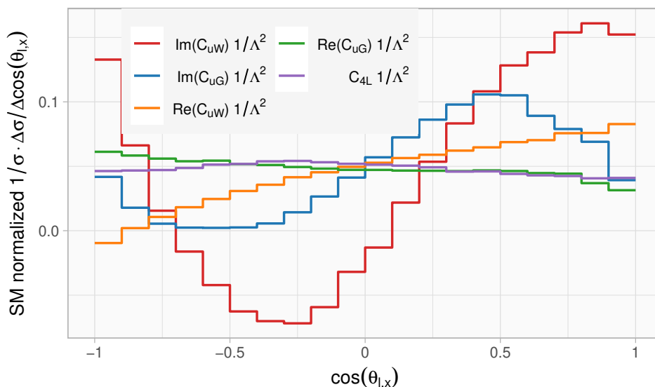
Figure 13. To itself and to the SM normalized SMEFT contributions to the \cos \theta_{l,x} distribution at NLO in QCD. Results are presented for the real and imaginary parts of \mathcal{C}_{uW}^{33} and \mathcal{C}_{uG}^{33} as well as for the four quark operator \mathcal{C}_{4L} .
