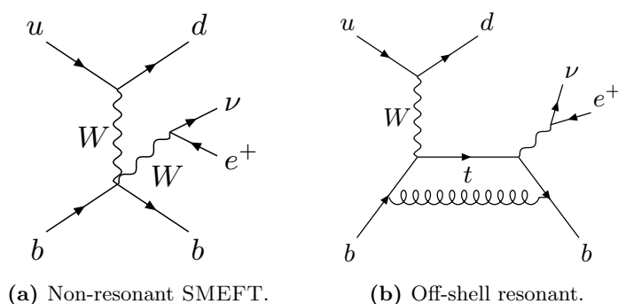
Figure 2. (a) Example non-resonant contribution in the SMEFT at LO. (b) One-loop resonant diagram with production-decay interference.
