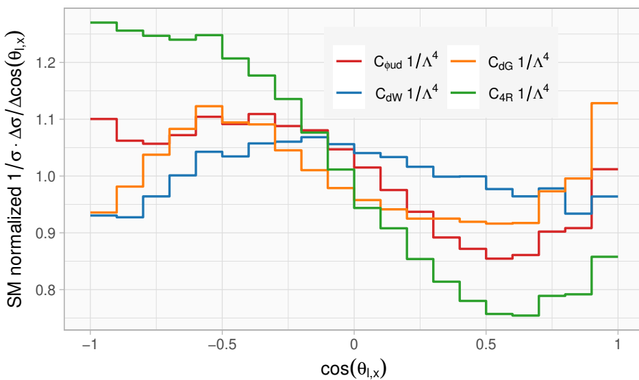
Figure 23. To itself and to the SM normalized SMEFT contributions to the \cos\theta_{l,x} distribution at NLO in QCD. Results are presented for Q_{\varphi ud}^{33} , Q_{dW}^{33} and Q_{dG}^{33} as well as for the four quark operator Q_{4R} .
