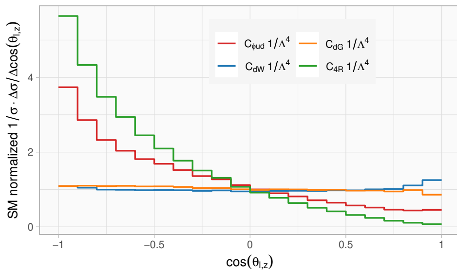
Figure 25. To itself and to the SM normalized SMEFT contributions to the \cos \theta_{l,z} distribution at NLO in QCD. Results are presented for Q_{\varphi ud}^{33} , Q_{dW}^{33} and Q_{dG}^{33} as well as for the four quark operator Q_{4R} .
