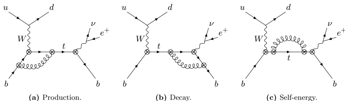
Figure 3. NLO virtual contribution to the (a) production vertex, (b) decay vertex, or (c) top-quark self-energy. Each crossed circle represents a possible SMEFT operator insertion.
