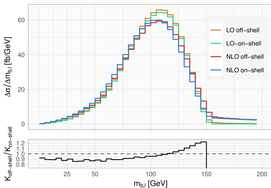
Figure 7. Invariant mass of the positron plus leading b -jet system for the top-quark on-shell approximation and for the off-shell top quark at LO and NLO. The lower panel shows the ratio of the NLO/LO K -factors from the off-shell and on-shell results.
