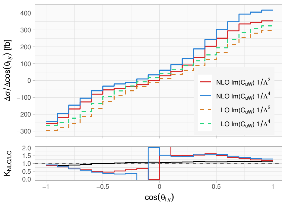
Figure 12. Distribution of \cos\theta_{l,y} for the pure SMEFT contribution with \Im m C_{uW}^{33} = 1 , \Lambda = 1000\text{ GeV} . Shown are results at LO and NLO in QCD and at 1/\Lambda^2 in the SMEFT as well as higher order effects 1/\Lambda^4 .
