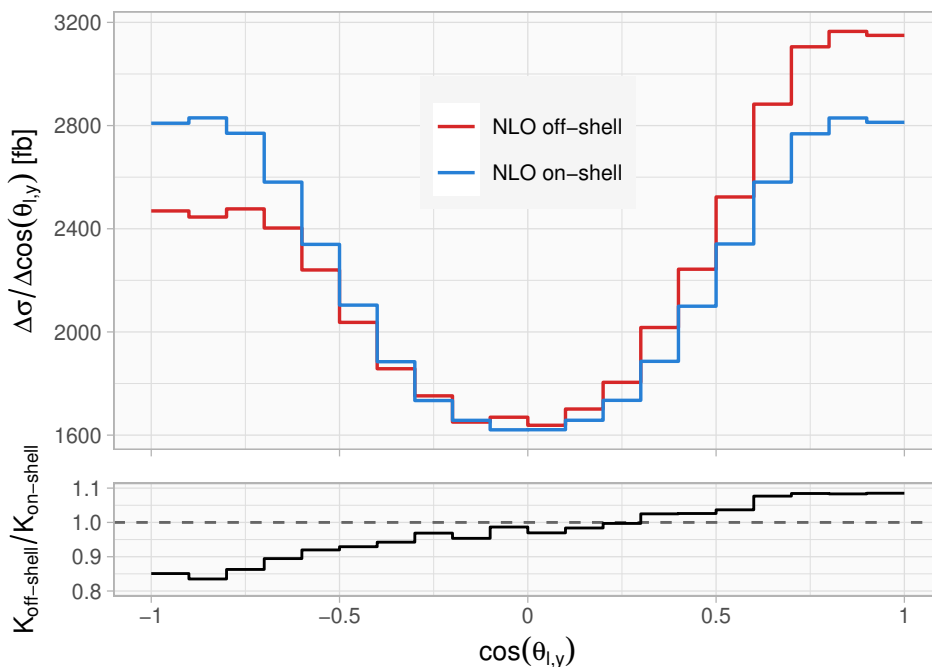
Figure 15. Distribution of \cos \theta_{l,y} at NLO in the on-shell approximation and for an off-shell top quark. The lower panel shows the ratio of the off-shell and on-shell K -factors. Note the range of the y -axis, which does not start at zero.
