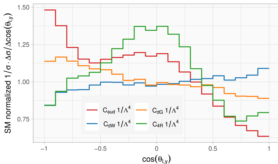
Figure 24. To itself and to the SM normalized SMEFT contributions to the \cos \theta_{l,y} distribution at NLO in QCD. Results are presented for Q_{\varphi ud}^{33} , Q_{dW}^{33} and Q_{dG}^{33} as well as for the four quark operator Q_{4R} .
