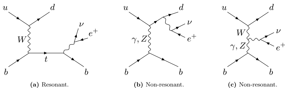
Figure 1. Sample Feynman diagrams of resonant and non-resonant contributions at LO.
