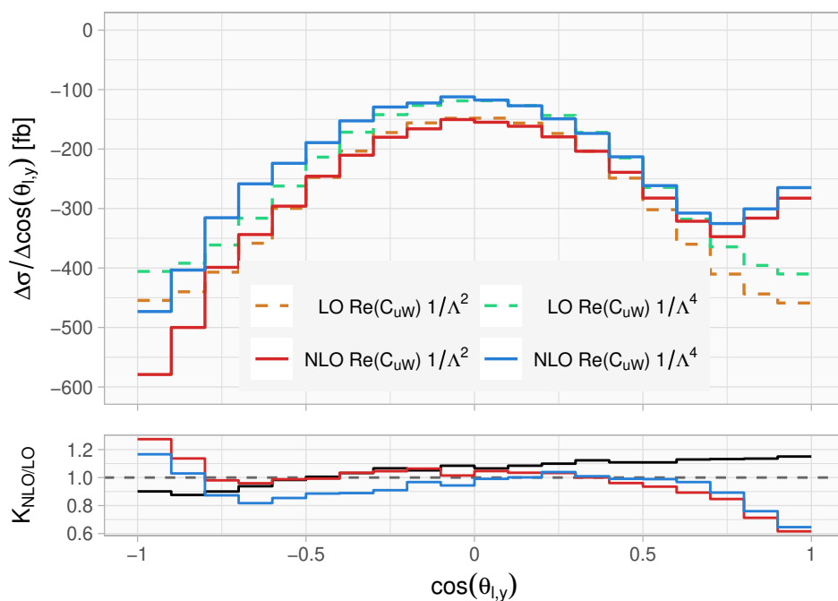
Figure 10. Distribution of \cos\theta_{l,y} for the pure SMEFT contribution with \Re c_{uW}^{33} = 1 , \Lambda = 1000 GeV. Shown are results at LO and NLO in QCD and at 1/\Lambda^2 in the SMEFT as well as with higher order effects 1/\Lambda^4 .
