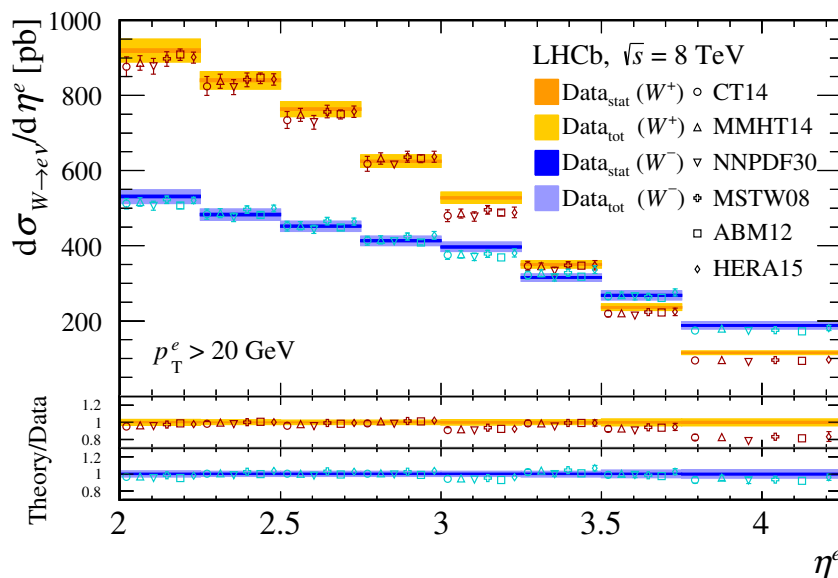
Figure 2. The differential W^+ and W^- cross-sections in bins of \eta^e . Measurements, represented as bands, are compared to NNLO predictions with different parameterisations of the PDFs (markers are displaced horizontally for presentation). The bottom panel displays the theory predictions divided by the measured cross-sections.
