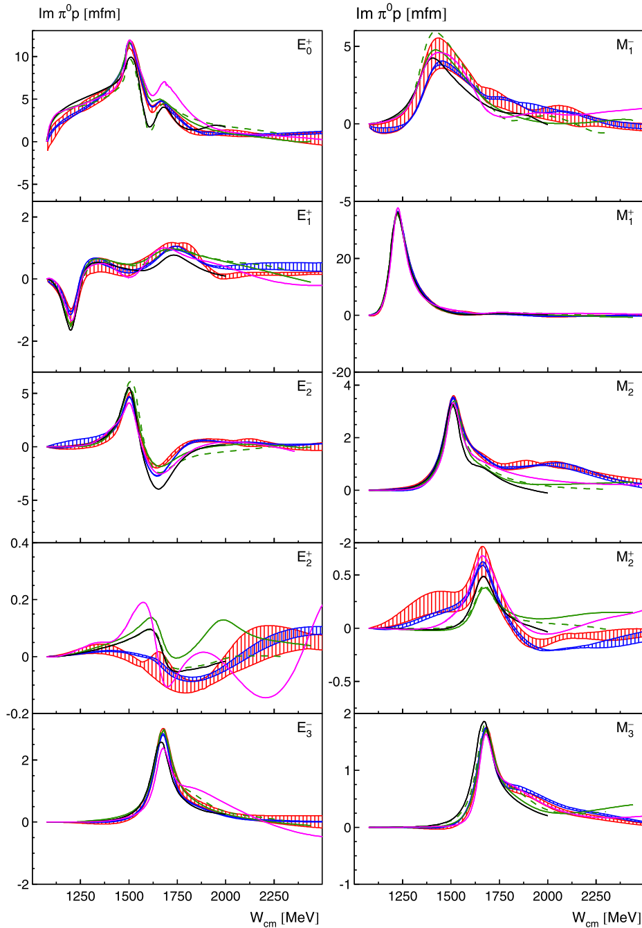
Fig. 10. (Color online.) Multipole decomposition of the \gamma p \rightarrow p\pi^0 transition amplitudes, imaginary part. The light (red) shaded areas give the range from a variety of different fits derived from solution BnGa2011-01 and BnGa2011-02 [5]. The dark (blue) shaded area represents the range of solutions when the new data are included in the fit. The black curves represent the MAID fit [3], the light (green) solid curves SAID-CM12 [22], the light (green) dashed curves SAID-SN11 [4], and the magenta curve the Jülich2015 [7] solution. For the BnGa-multipoles an error band (see text) has been determined. Such an error band is presently not provided by the other analyses.
