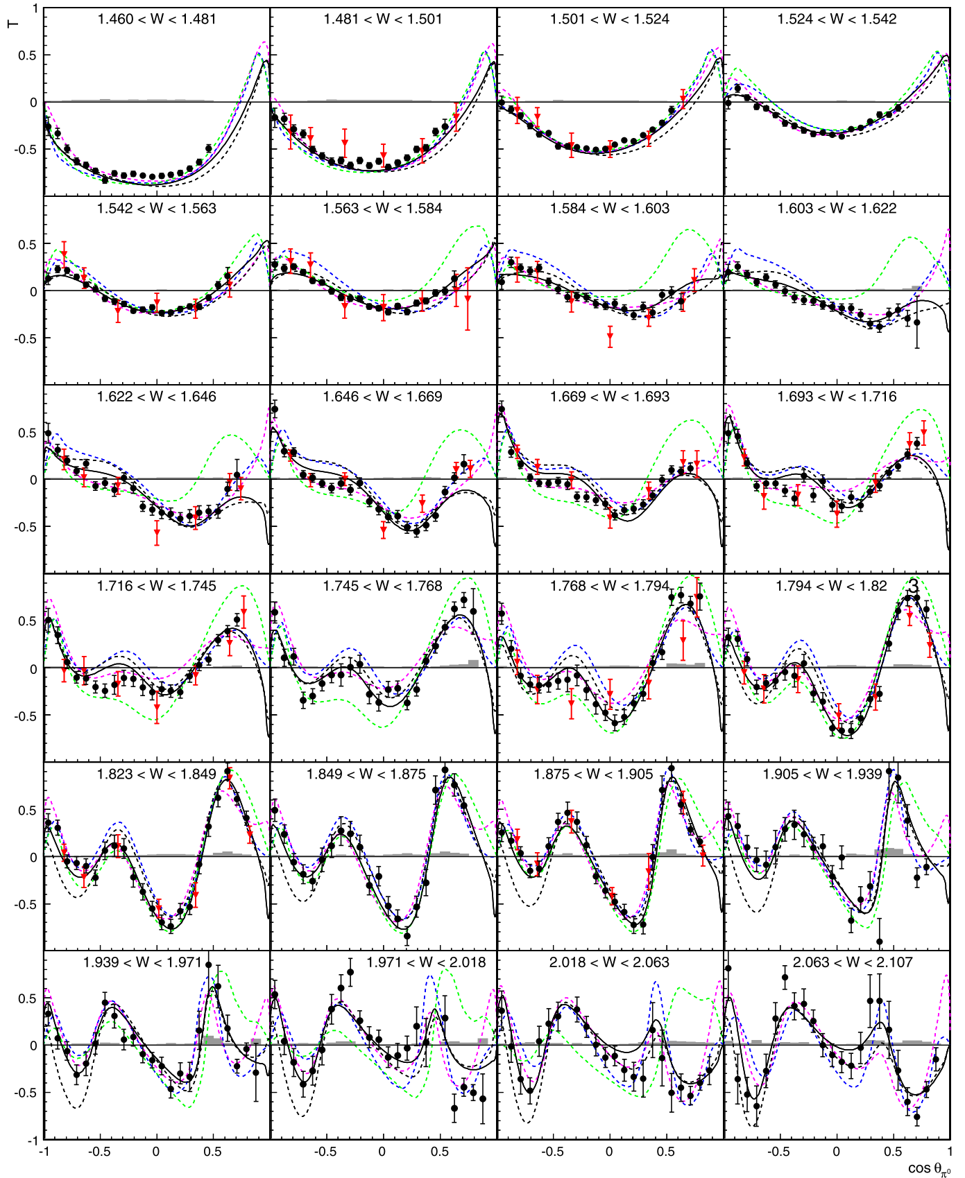
Fig. 7. (Color online.) The polarization observable T as function of the \gamma p invariant mass W (in GeV) and of the scattering angle \cos\theta . The systematic uncertainty is shown as dark gray band. An additional systematic uncertainty on the photon energy (from \sigma_{E_\gamma}^{\text{sys}} = 6.5 MeV at the lowest to 2.3 MeV at the highest energy bin) is not shown. The low energy data were presented in [6]. Earlier data (gray, (red, online)) are from [20]. The solid line represents our best fit BnGa2014. The data are compared to predictions (dashed curves) from BnGa2011-02 (black), MAID [3] (light gray, (green, online)), SAID CM12 [22] (dark gray, (blue, online)), and Jülich2015 [7] (gray, (magenta, online)).
