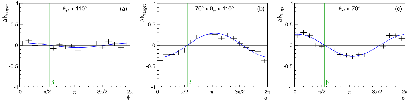
Fig. 5. (Color online.) Yield asymmetry \Delta N_{\text{target}} as a function of \phi for three angular bins in \theta in the \gamma p invariant mass window 1.82 \text{ GeV} < W < 1.94 \text{ GeV} .
