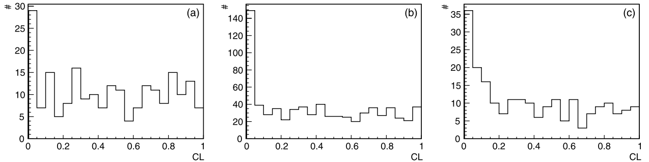
Fig. 6. Histograms of the confidence level of the fits to the (a) \Delta N_{\text{beam}}(\phi) , (b) \Delta N_{\text{target}}(\phi) , and (c) \Delta N_{\text{beam-target}}(\phi) distributions. The increase of the CL in the first bin can be eliminated by requiring \text{CL} > 0.001 .
