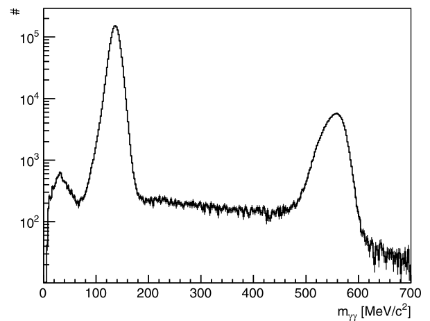
Fig. 2. The invariant \gamma\gamma mass distribution for the butanol data, after all cuts discussed (see text) have been applied. The final data sample of p\pi^0 events has a background contamination of less than 1%.
