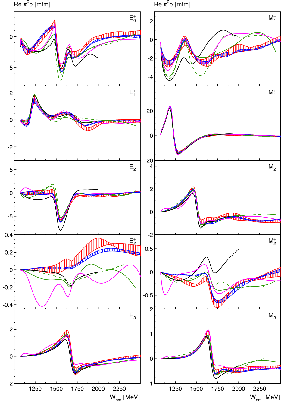
Fig. 11. (Color online.) Multipole decomposition of the \gamma p \rightarrow p\pi^0 transition amplitudes, real part. The light (red) shaded areas give the range from a variety of different fits derived from solution BnGa2011-01 and BnGa2011-02 [5]. The dark (blue) shaded area represents the range of solutions when the new data are included in the fit. The black curves represent the MAID fit [3], the light (green) solid curves SAID-CM12 [22], the light (green) dashed curves SAID-SN11 [4], and the magenta curve the Jülich2015 [7] solution. For the BnGa-multipoles an error band (see text) has been determined. Such an error band is presently not provided by other analyses.
