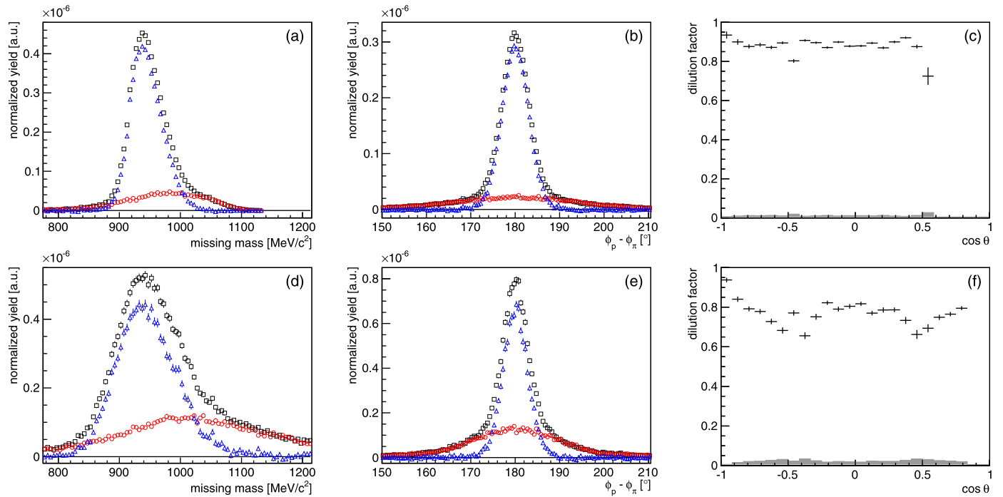
Fig. 3. (Color online.) (a, d) The missing mass distribution, with the proton as the missing particle, and (b, e) the azimuthal angle difference of \pi^0 and proton for reaction (1), for a \gamma p invariant mass of W = 1.46\text{--}1.48 (top) and 1.82\text{--}1.94 GeV (bottom); butanol ( \square ), scaled carbon ( \circ ), and the difference ( \triangle ). The distributions are shown after all other cuts discussed in the text are applied. From these distributions, the dilution factor (c, f) is determined. The gray band indicates the systematic uncertainty in the dilution factor due to uncertainties in the determination of the carbon scaling factor s . Since only events with all three particles detected in the calorimeter are considered an acceptance hole occurs for large \cos\theta . The observed structures in the dilution factor are due to a combined effect of reduced efficiencies for clusters impinging onto detector boundaries and Fermi smearing.
