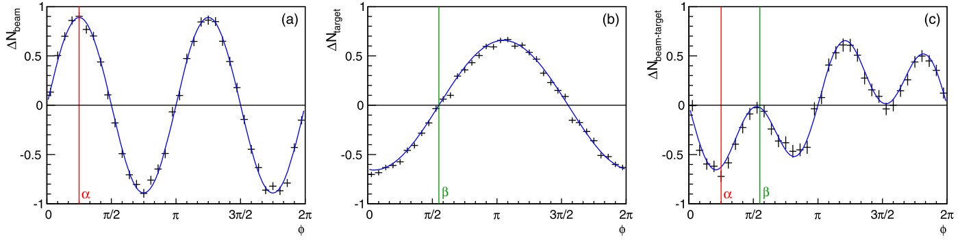
Fig. 4. (Color online.) Yield asymmetries as a function of \phi for the energy bin 1.46 \text{ GeV} < W < 1.48 \text{ GeV} . (a) \Delta N_{\text{beam}}(\phi) , (b) \Delta N_{\text{target}}(\phi) , (c) \Delta N_{\text{beam-target}}(\phi) fitted by the function of Eq. (5), Eq. (6), and Eq. (7), respectively.
