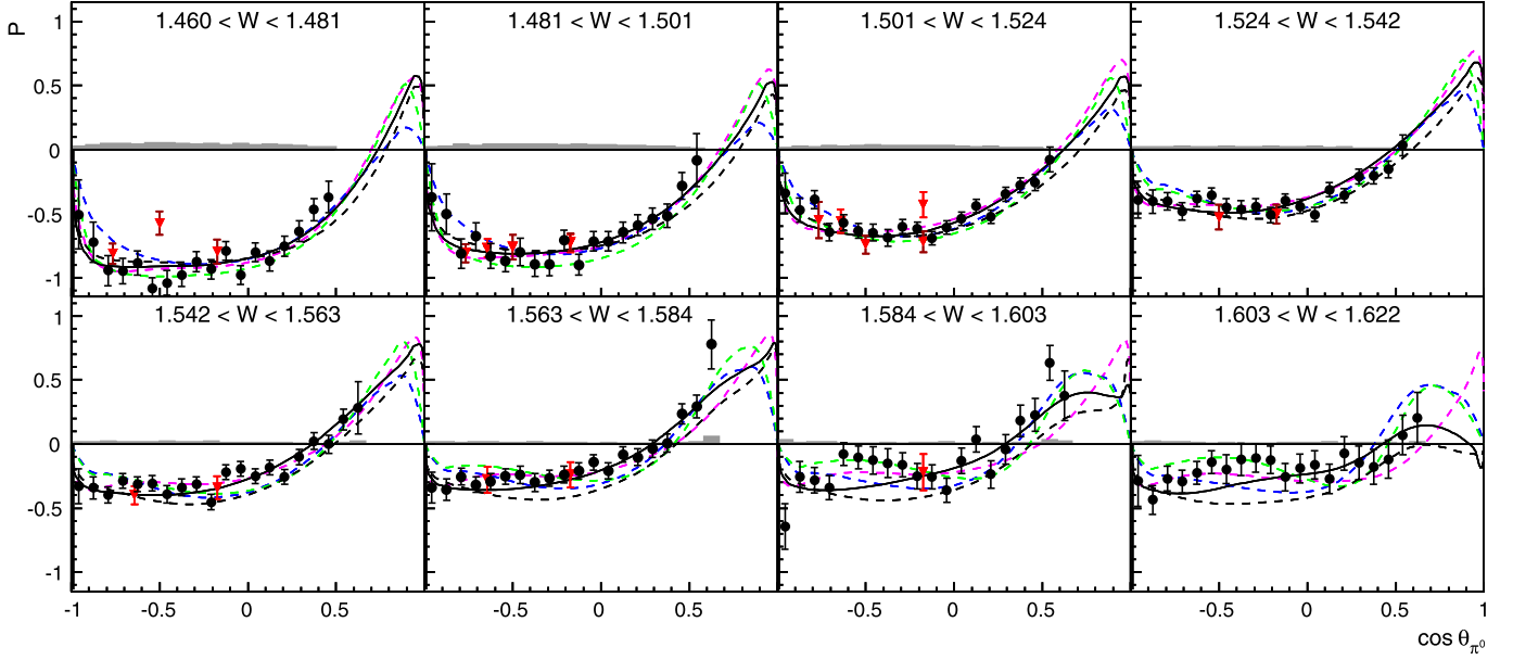
Fig. 8. (Color online.) The polarization observable P [6] as functions of the \gamma p invariant mass W (in GeV) and of the scattering angle \cos\theta . The systematic uncertainty is shown as dark gray band. An additional systematic uncertainty on the photon energy (from \sigma_{E_\gamma}^{\text{sys}} = 6.5 MeV at the lowest to 5.4 MeV at the highest energy bin) is not shown. Earlier data (gray, (red, online)) are from [19]. The solid line represents our best fit BnGa2014. The data are compared to predictions (dashed curves) from BnGa2011-02 (black), MAID [3] (light gray, (green, online)), SAID CM12 [22] (dark gray, (blue, online)), and Jülich2015 [7] (gray, (magenta, online)).
