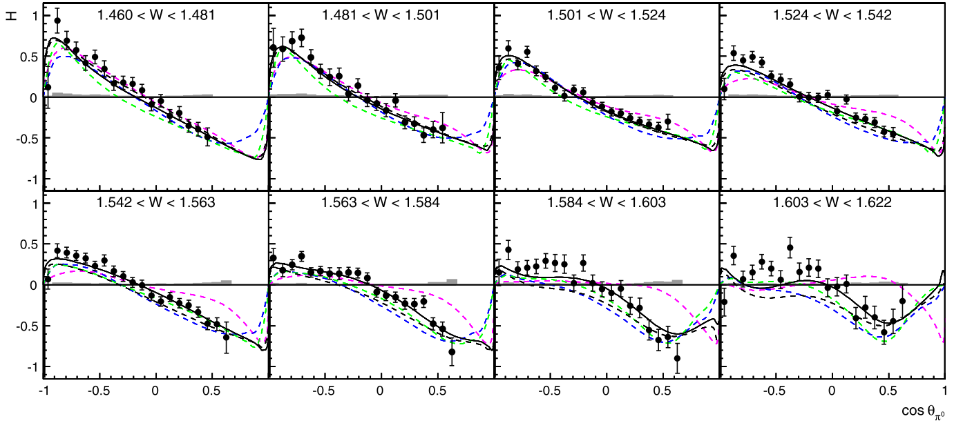
Fig. 9. (Color online.) The polarization observable H [6] as functions of the \gamma p invariant mass W (in GeV) and of the scattering angle \cos\theta . The systematic uncertainty is shown as dark gray band. An additional systematic uncertainty on the photon energy (from \sigma_{E_\gamma}^{\text{sys}} = 6.5 MeV at the lowest to 5.4 MeV at the highest energy bin) is not shown. The data are compared to predictions (dashed curves) from BnGa2011-02 (black), MAID [3] (light gray, (green, online)), SAID CM12 [22] (dark gray, (blue, online)), and Jülich2015 [7] (gray, (magenta, online)).
