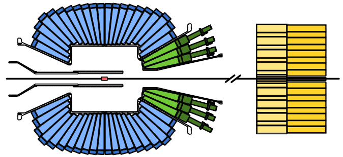
Fig. 1. (Color online.) The central part of the detector system. The 1320 CsI(Tl) crystals (blue and green) are read out via wavelength shifters and photodiodes (blue) or via photomultipliers (green), the 216 BaF 2 crystals (yellow) in forward direction are read out with photomultipliers. The target is surrounded by a 3-layer-scintillating fiber detector. To detect charged particles, scintillators are also placed in front of the forward CsI(Tl) (green) and TAPS crystals (yellow).
