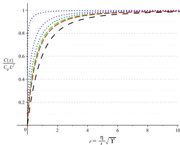
Figure 1 (b). Plot of the c -function in terms of the canonical radial coordinate r = \frac{\eta\sqrt{\Upsilon}}{L} = \frac{\eta}{L} \frac{\nu x^{\nu-1}}{x^{\nu-1}} for the same values of the \nu parameter.
