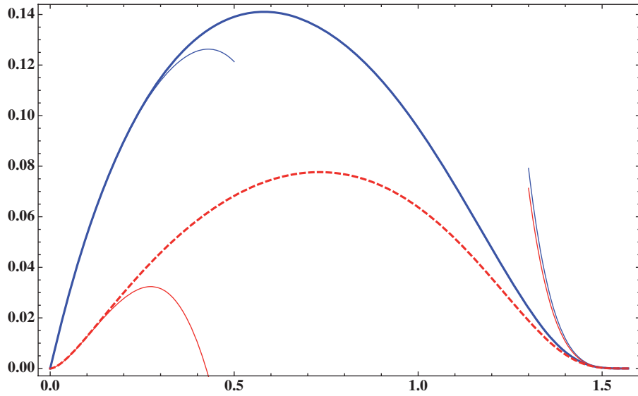
Fig. 2. \delta\Lambda(m\tau)/\Lambda_\tau(m\tau) as a function of m\tau at d = 3 (blue solid line) and d = 4 (red dashed line), where the horizontal axis is x = \arctan(m\tau) , together with asymptotic behaviors at UV ( x \simeq 0 ) and IR ( x \simeq \pi/2 ).
