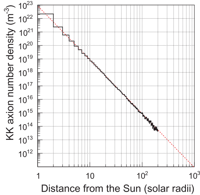
Fig. 1. Number density of trapped KK axions against the distance from the Sun. The black solid histogram shows the simulated distribution taken from Ref. [8] with g_{a\gamma\gamma} = 9.2 \times 10^{-14} \text{ GeV}^{-1} . The red dotted line shows the fitted r^{-4} curve. The unit of distance is the radius of the Sun (695,700 km). Using this unit, the distance between the Earth and the Sun is 211.4R_{\odot} at perihelion and 218.6R_{\odot} at aphelion.
