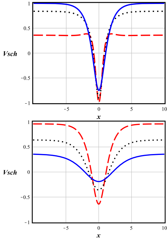
Fig. 6. Schrödinger-like potential V_{sch}(x) . (a) (upper) The figures are for fixed A = 0.1 (red dash), A = 0.3 (black dotted), A = 0.5 (blue solid). (b) (bottom) The figures are for fixed A = 0.6 (red dash), A = 0.8 (black dotted), A = 0.9 (blue solid). Note that there is a transition around A \sim 0.5 . See also Fig. 5.
