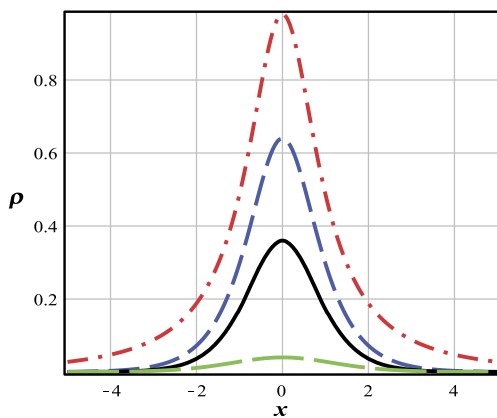
Fig. 3. The energy density \rho(x) . The figures are for fixed A = 0.01 (red dash-dot), A = 0.2 (blue dashed), A = 0.4 (black line) and A = 0.8 (green long-dash).
