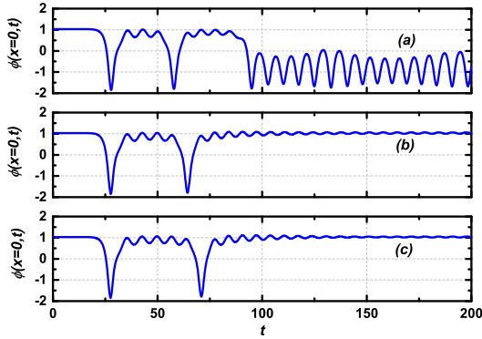
Fig. 11. Scalar field at the center of mass \phi(0, t) versus time for fixed A = 0.4 and (a) v_i = 0.5398 , (b) v_i = 0.5441 and (c) v_i = 0.5464 .
