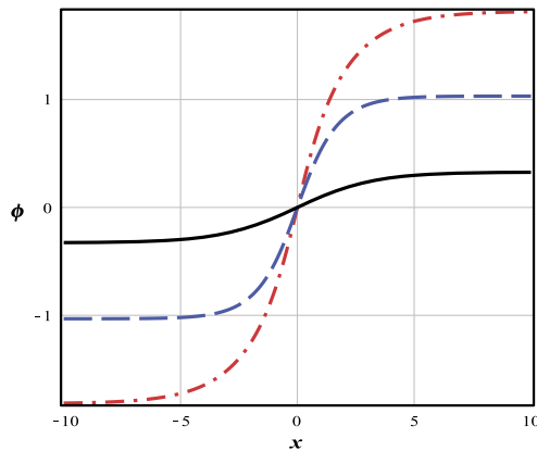
Fig. 2. Field configurations \phi(x) . The figures are for fixed A = 0.1 (red dash-dotted), A = 0.4 (blue dash), A = 0.9 (black line).
