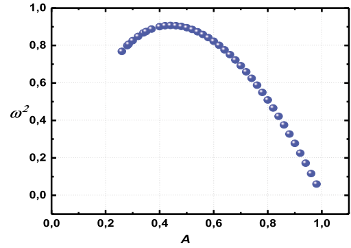
Fig. 7. Squared frequency \omega^2 for the vibrational state as a function of A . The curve has a maximum at A = 0.44 . See also Fig. 5.
