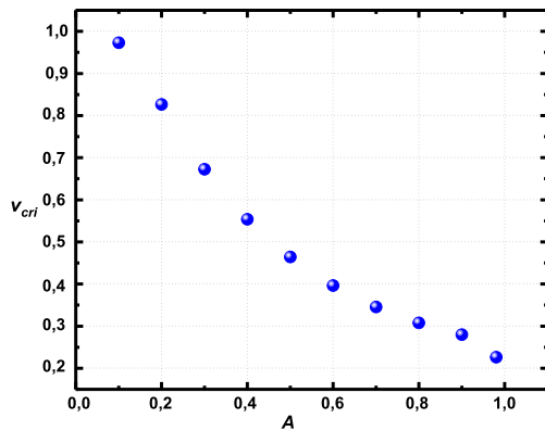
Fig. 9. Critical velocity as a function of A .
