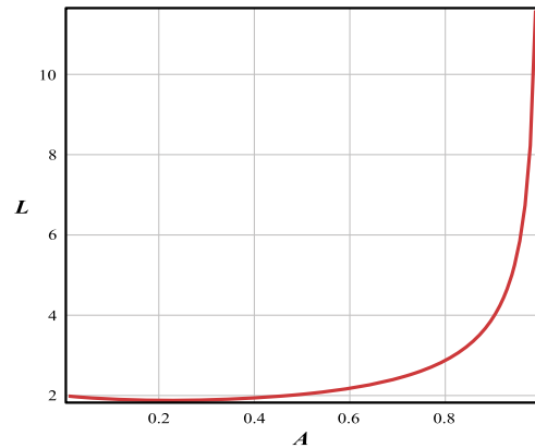
Fig. 4. Kink width L as a function of A . Note the minimum around A \simeq 0.22 . See also Fig. 5.
