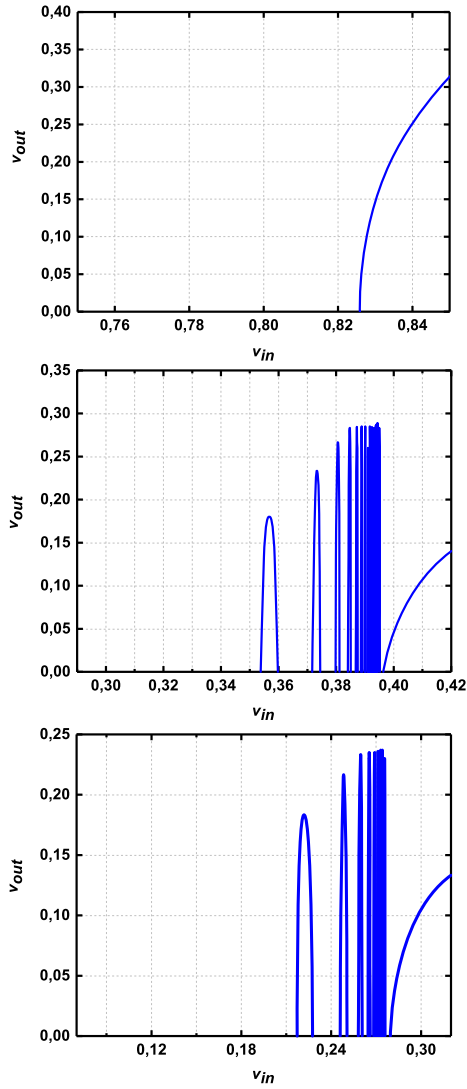
Fig. 8. The output (final) kink velocity after a K\bar{K} collision as a function of input (initial) velocities for a) A = 0.2 , b) A = 0.6 and c) A = 0.9 .
