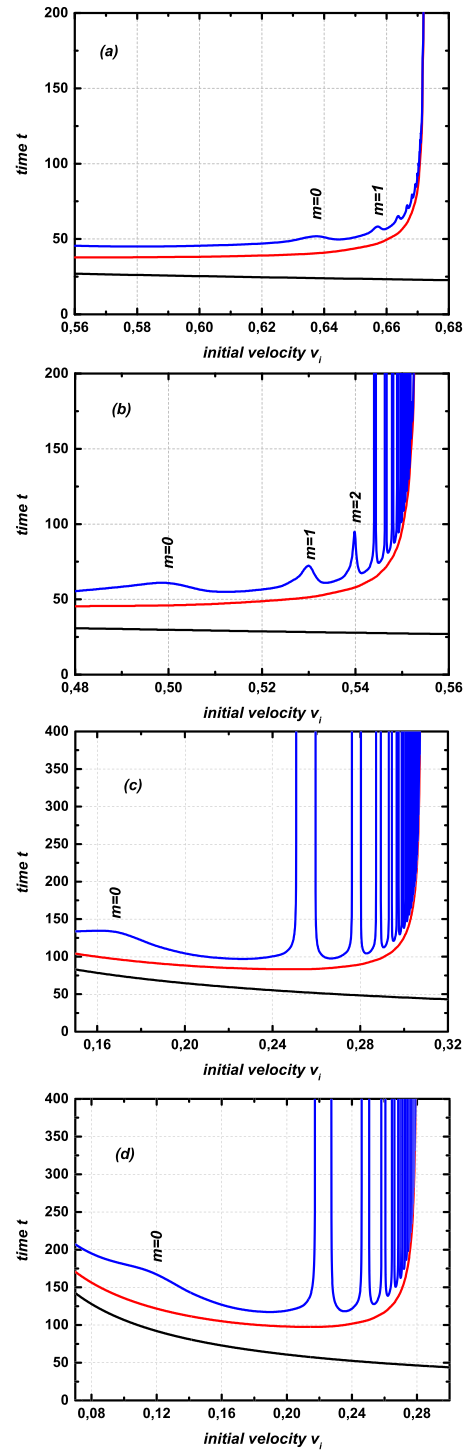
Fig. 10. Times to the first (black), second (red) and third (blue) kink–antikink collisions as a function of initial velocity v_i for a) A = 0.3 , b) A = 0.4 , c) A = 0.8 , d) A = 0.9 . Some peaks include also the number m of oscillations between bounces for the observed false two-bounce windows. (For interpretation of the references to color in this figure legend, the reader is referred to the web version of this article.)
