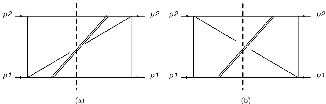
Figure 1. Phase space integrals contributing to triple real corrections to Higgs boson production at N^3\text{LO} . The computation of these integrals involves elliptic integrals. Solid lines represent Feynman propagators. Solid lines crossed by the dashed line correspond to cut-propagators. The doubled line represents the on-shell constraint of the Higgs boson.
