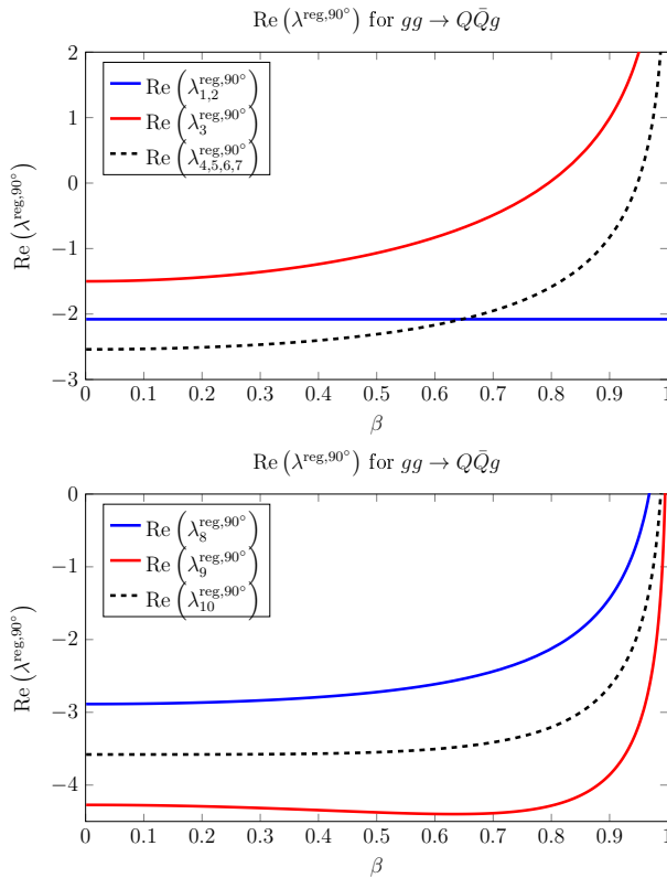
Fig. 5. The real parts of the regularized eigenvalues of \tilde{T}_S for gg \rightarrow Q\bar{Q}g at \theta = 90^\circ .
