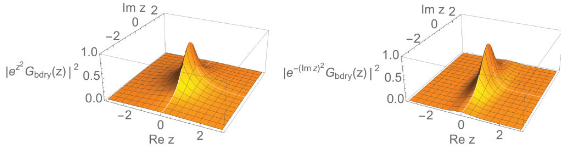
Fig. 2. Normalized boundary function |e^{z^2} G_{\text{bdry}}(z)|^2 (left) and the combination that appears in the physical setup |e^{-(\Im z)^2} G_{\text{bdry}}(z)|^2 (right).
