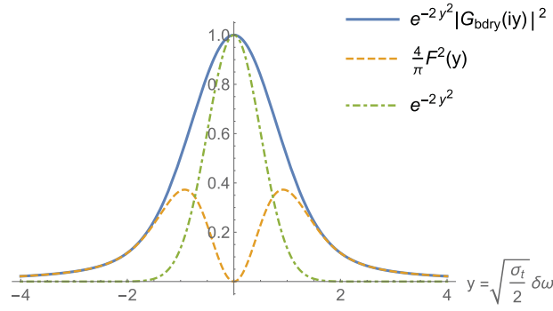
Fig. 3. e^{-2y^2} |G_{\text{bdry}}(iy)|^2 (solid), \frac{4}{\pi} F^2(y) (dashed), and e^{-2y^2} (dot-dashed) as a function of y = \sqrt{\frac{\sigma_t}{2}} \delta\omega , which corresponds to right on either boundary \mathfrak{T} = T_{\text{in/out}} . The solid line is the sum of the dashed and dot-dashed lines and corresponds to the ridge line at \Re z = 0 in Fig. 2.
