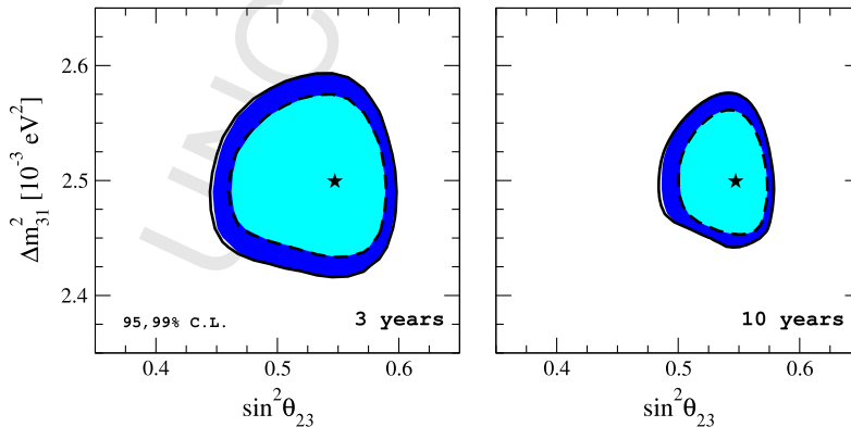
Fig. 4. ORCA sensitivity to the atmospheric oscillation parameters in the standard picture (filled regions) and with neutrino decay after marginalizing over \alpha_3 (black lines) at 95% and 99% C.L. after 3 years (left panel) and 10 years (right panel) of running time.
