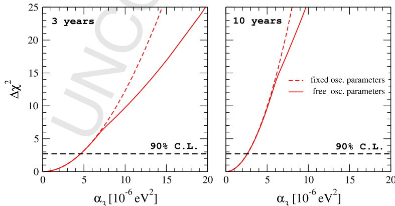
Fig. 3. Sensitivity of ORCA to the neutrino decay constant \alpha_3 . Solid (dashed) lines correspond to the analysis with free (fixed) oscillation parameters \Delta m_{31}^2 and \theta_{23} . The left (right) panel shows the results for three (ten) years of operational time.
