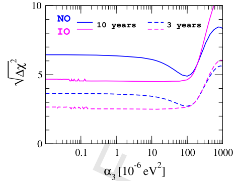
Fig. 5. ORCA sensitivity to the neutrino mass ordering as a function of the decay constant \alpha_3 . Blue (magenta) lines correspond to the case in which the true ordering is assumed to be normal (inverted), and solid (dashed) lines correspond to an exposure time of 10 years (3 years).
