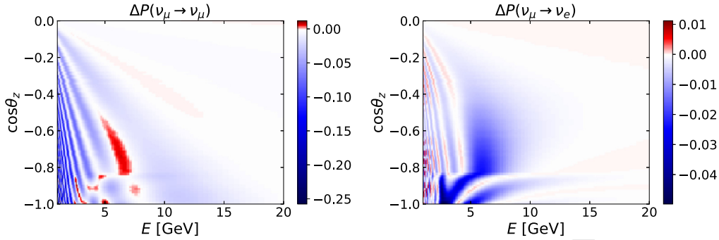
Fig. 1. Differences in the oscillation probability of atmospheric muon neutrinos with and without decay, \Delta P = p^{\text{decay}} - p^{\text{standard}} , for the \nu_\mu \rightarrow \nu_\mu (left panel) and \nu_\mu \rightarrow \nu_e (right panel) oscillation channels. A value of \alpha_3 = 10^{-5} \text{ eV}^2 has been assumed in both cases. The difference in the probabilities is shown as a function of the neutrino energy and arrival zenith angle.
