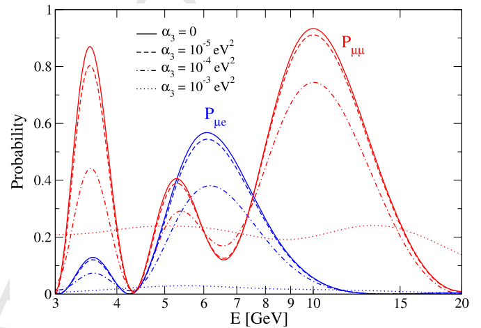
Fig. 2. Muon neutrino survival probability, P_{\mu\mu} , and electron neutrino appearance probability, P_{\mu e} , as a function of the energy for the arrival direction \cos\theta_z = -0.82 . The solid lines correspond to the standard case, without neutrino decay, while the dashed, dashed-dotted and dotted lines have been obtained assuming \alpha_3 = 10^{-5} , 10^{-4} and 10^{-3} \text{ eV}^2 , respectively.
