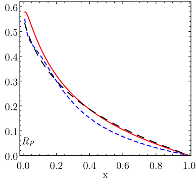
FIG. 6. Power correction to the pPDF \mathcal{R}_P (68) for MSTW valence u-quarks (long black dashes), d-quarks (short blue dashes), both at 2 GeV, and for the simple model q(x) = x^{-1/2}(1-x)^3 (red solid curve).
