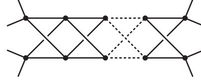
FIG. 5. Massless, finite four-dimensional Feynman integrals with rigidity 2(L - 1) for odd L \geq 5 .
