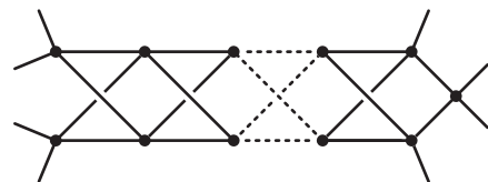
FIG. 3. Massless, finite four-dimensional Feynman integrals with rigidity 2(L - 1) for even L \geq 2 .
