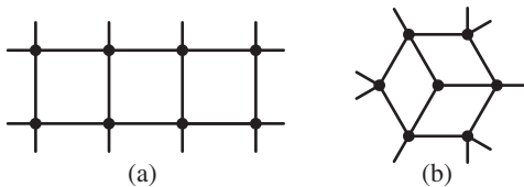
FIG. 6. The two most rigid three-loop integrals in the planar limit: (a) the traintrack with rigidity 2 and (b) a diagram with rigidity 3.
