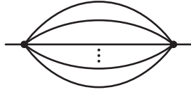
FIG. 1. The marginal, L -loop sunrise integral in two dimensions. It has (maximal) rigidity (L - 1) iff all legs are massive.
