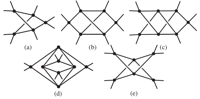
FIG. 2. Examples of (a) two-, (b) three-, (c) four-, and (d) five-loop marginal integrals with maximal rigidity; (e) a marginal integral with submaximal rigidity.
