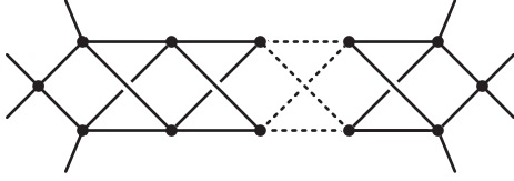
FIG. 4. Massless, finite four-dimensional Feynman integrals with rigidity 2(L - 1) for odd L \geq 1 .
