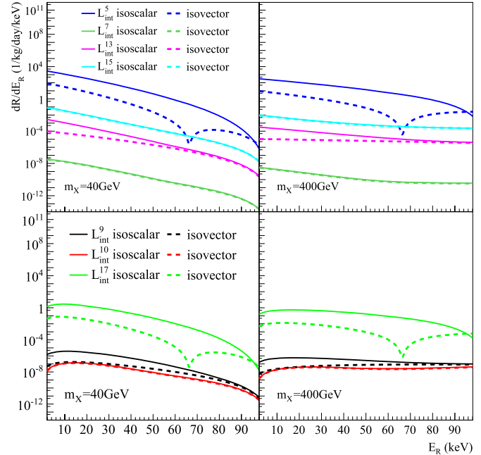
Fig. 1. Recoil energy spectra for the scattering of spin- \frac{1}{2} WIMPs on xenon nuclei, for WIMP masses of 40 \text{ GeV}/c^2 and 400 \text{ GeV}/c^2 , and unit isoscalar ( d_i^0 = 1, d_i^1 = 0 ) and isovector ( d_i^0 = 0, d_i^1 = 1 ) coupling. Top panel: dimension-four V-A interactions. Bottom panel: higher dimension magnetic and electric dipole interactions.
