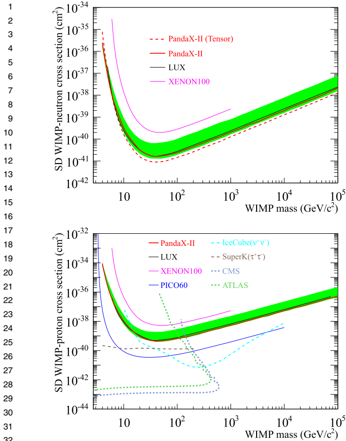
Fig. 4. PandaX-II exclusion limits on the WIMP-nucleon cross section for the standard SD interaction assuming neutron-only (top panel) and proton-only (bottom panel) coupling. The 1\sigma sensitivity bands are shown in green. Also shown are recent results from LUX [5], XENON100 [9], ATLAS [31], CMS [32], PICO-2L [33], PICO-60 [34,35], IceCube [36] and Super-K [37]. The dashed line (top panel) gives PandaX-II limits on tensor WIMP-neutron couplings.
