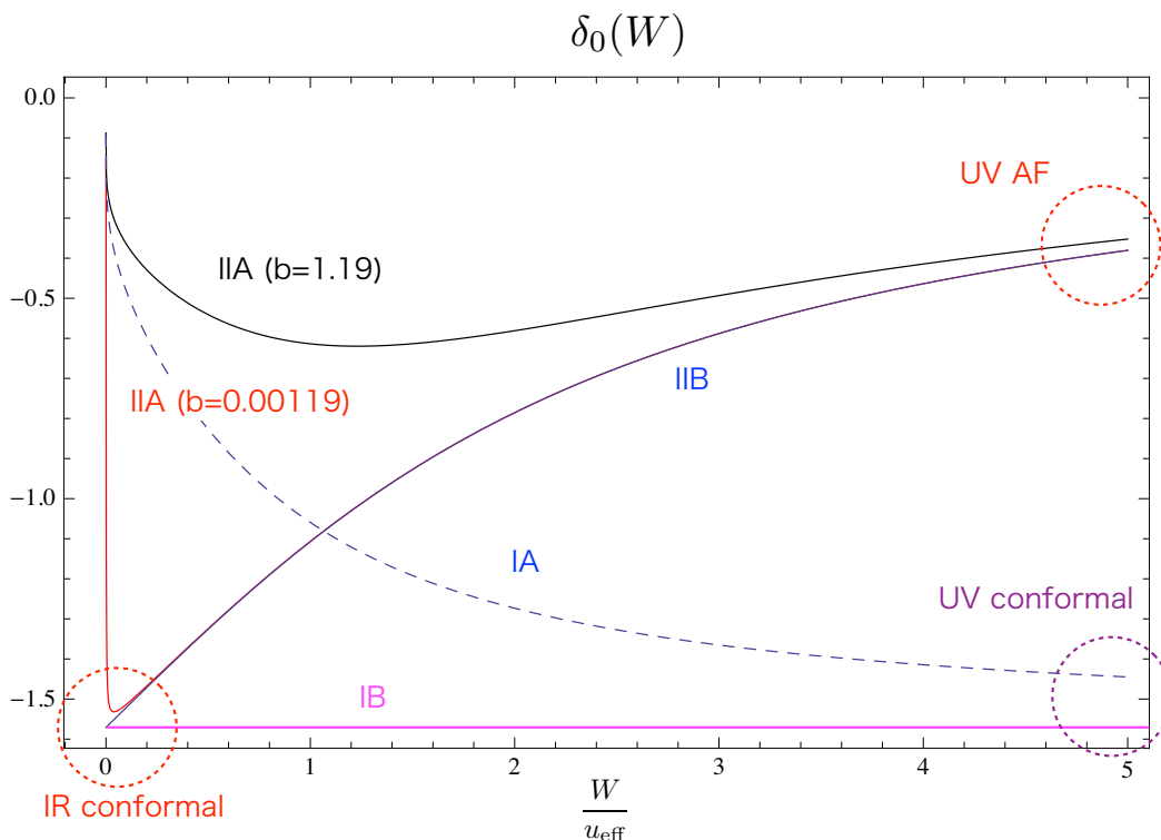
Figure 4. Scattering phase shift \delta_0(W) as a function of W/u_{\text{eff}} for IA(dashed line), IB(solid magenta line), IIA with b = 96\alpha = 1.19 (solid black line), IIA with b = 0.00119 (solid red line) and IIB (solid blue line).
