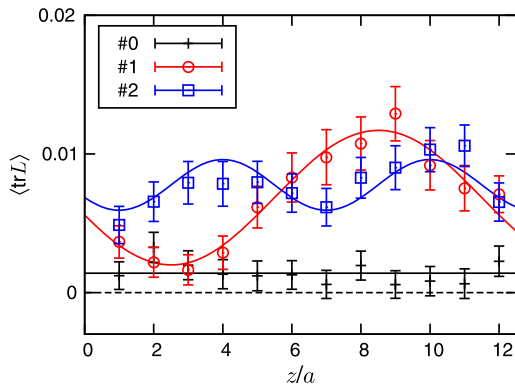
Fig. 2. Spatial distribution of the Polyakov loop. Three types of data correspond to three types of the backgrounds in Fig. 1. The solid curves are drawn for guide for eyes.
